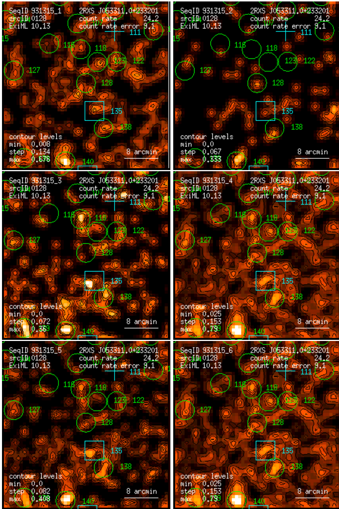
Figure 128: RASS 931315: detection 0128: band rate images, Gaussian filter: (1) PSPC channels 11 – 41, (2) 52 – 90, (3) 91 – 201, (4) 11 – 235, (5) 52 – 201, (6) 11 – 201. Broad band rates in counts/ks. Band rate contour levels in counts/ks/arcmin 2 .
