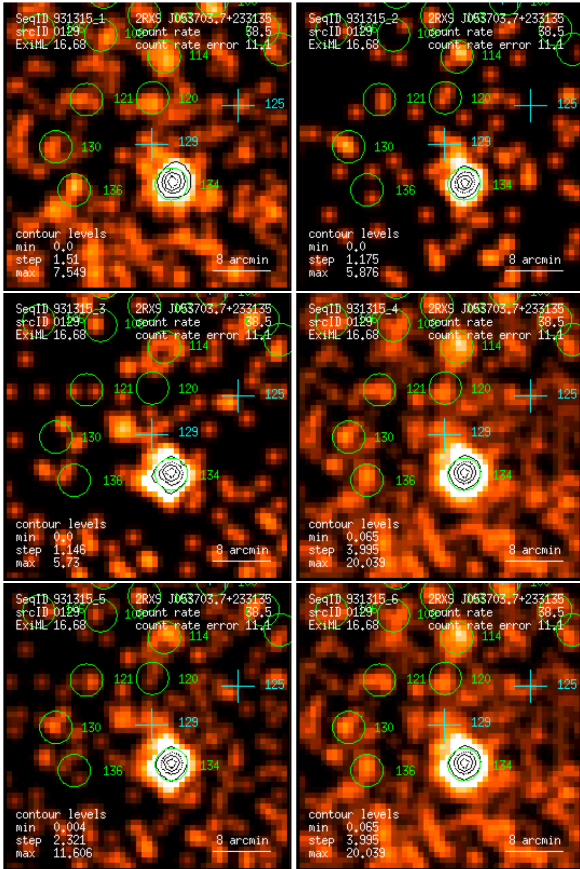
Figure 129: RASS 931315: detection 0129: band rate images, Gaussian filter: (1) PSPC channels 11 – 41, (2) 52 – 90, (3) 91 – 201, (4) 11 – 235, (5) 52 – 201, (6) 11 – 201. Broad band rates in counts/ks. Band rate contour levels in counts/ks/arcmin 2 .
