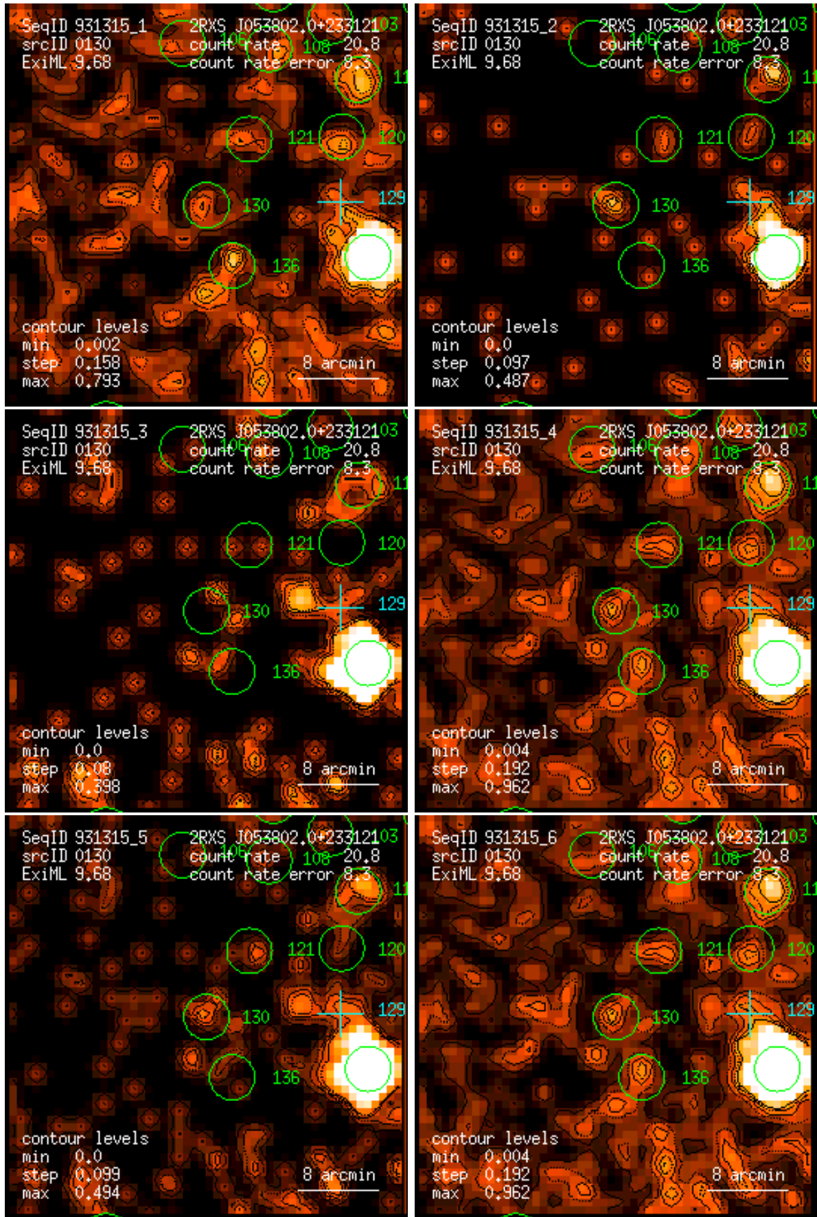
Figure 130: RASS 931315: detection 0130: band rate images, Gaussian filter: (1) PSPC channels 11 – 41, (2) 52 – 90, (3) 91 – 201, (4) 11 – 235, (5) 52 – 201, (6) 11 – 201. Broad band rates in counts/ks. Band rate contour levels in counts/ks/arcmin 2 .
