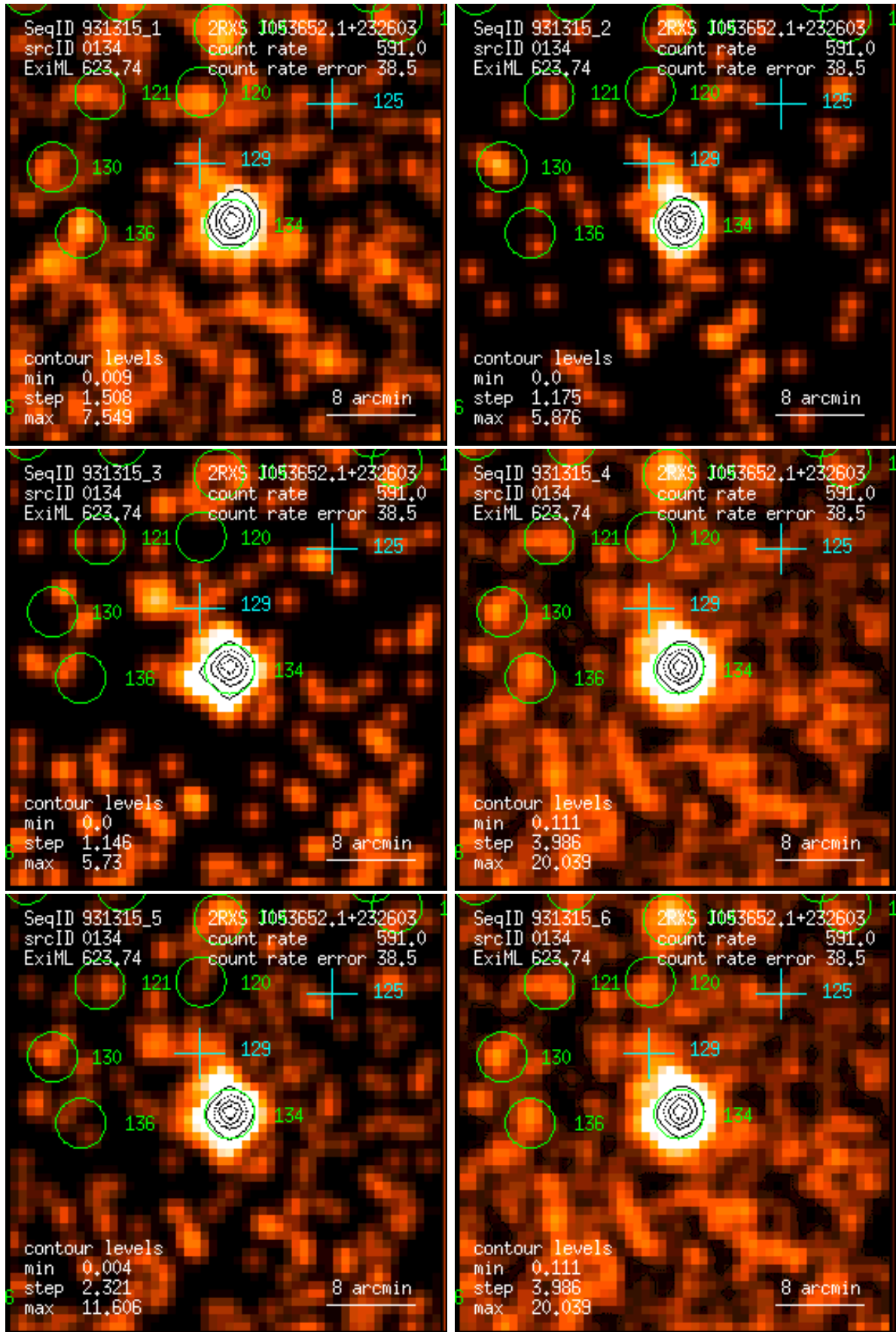
Figure 134: RASS 931315: detection 0134: band rate images, Gaussian filter: (1) PSPC channels 11 – 41, (2) 52 – 90, (3) 91 – 201, (4) 11 – 235, (5) 52 – 201, (6) 11 – 201. Broad band rates in counts/ks. Band rate contour levels in counts/ks/arcmin 2 .
