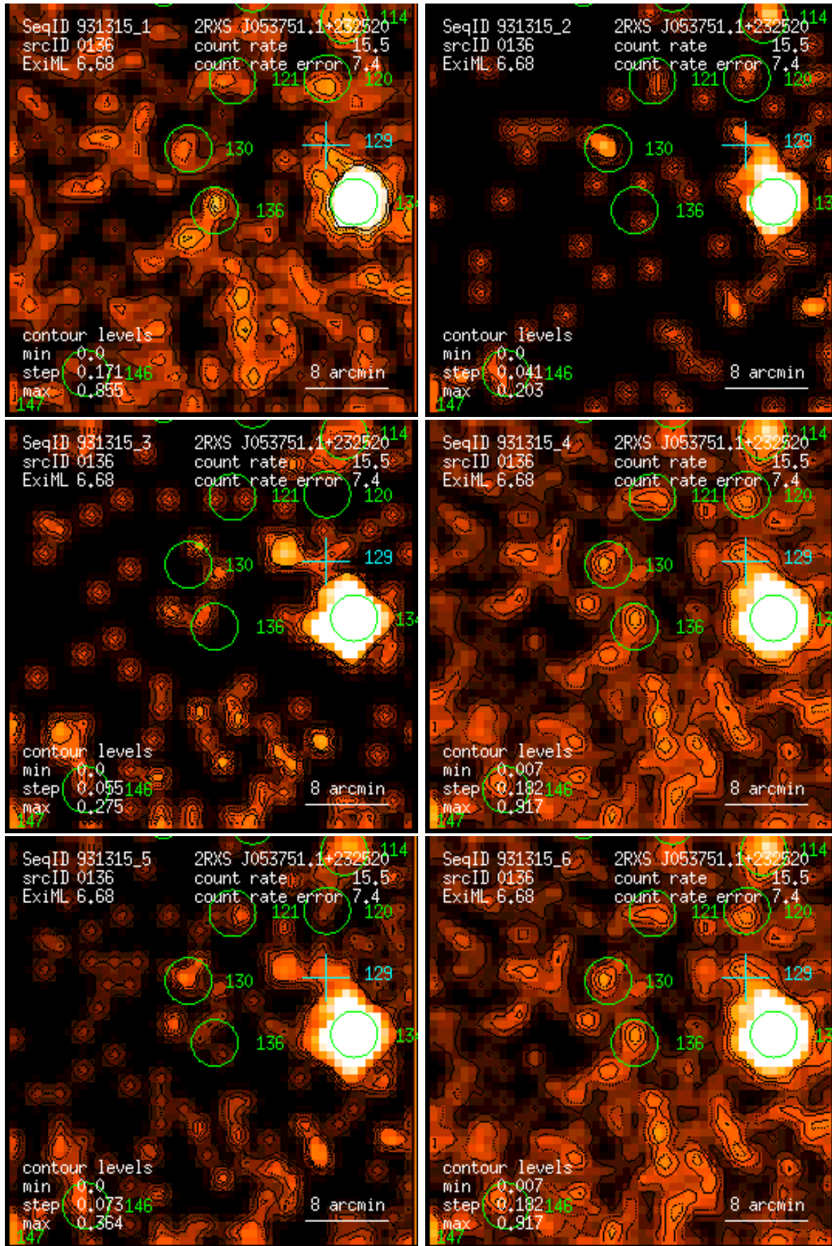
Figure 136: RASS 931315: detection 0136: band rate images, Gaussian filter: (1) PSPC channels 11 – 41, (2) 52 – 90, (3) 91 – 201, (4) 11 – 235, (5) 52 – 201, (6) 11 – 201. Broad band rates in counts/ks. Band rate contour levels in counts/ks/arcmin 2 .
