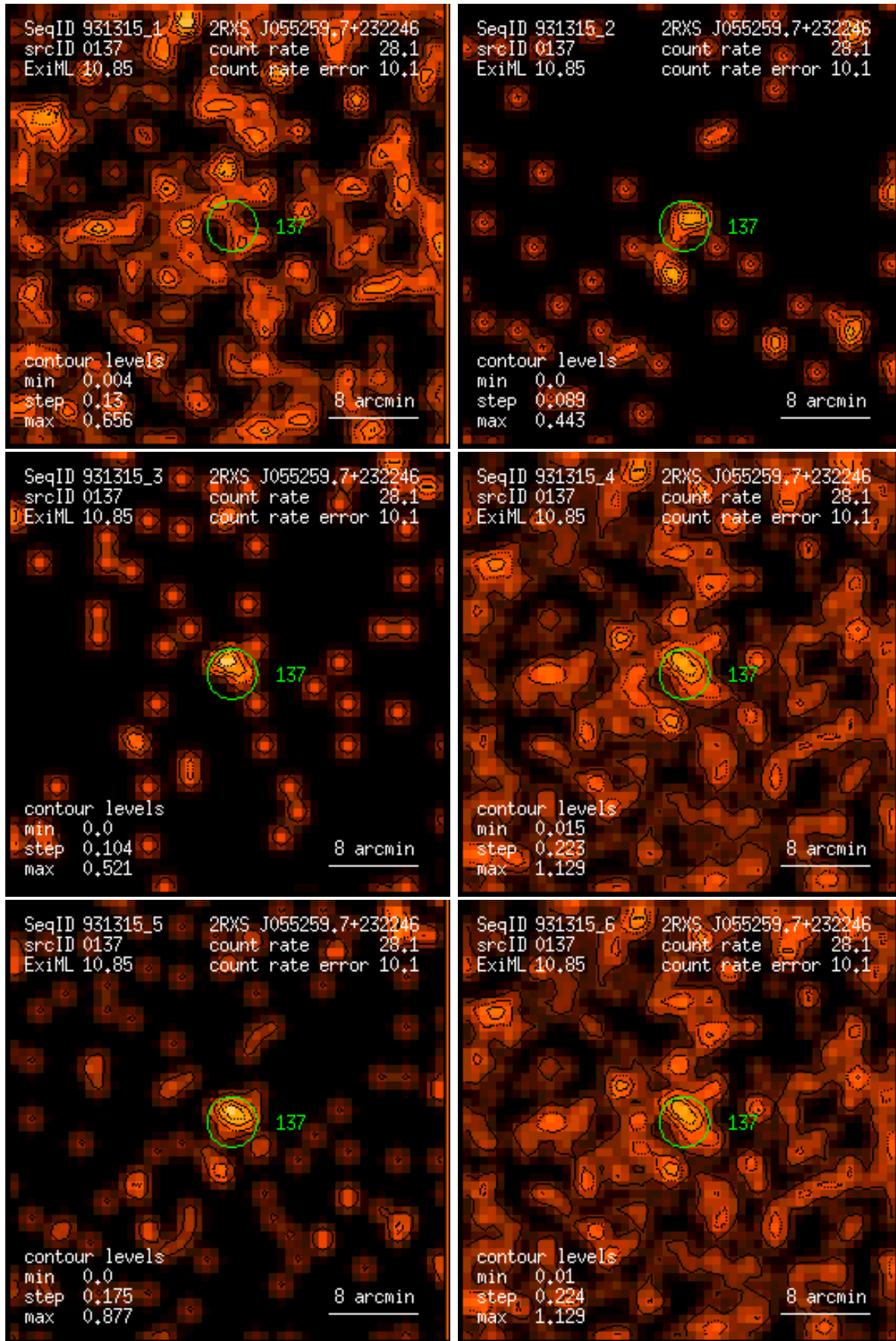
Figure 137: RASS 931315: detection 0137: band rate images, Gaussian filter: (1) PSPC channels 11 – 41, (2) 52 – 90, (3) 91 – 201, (4) 11 – 235, (5) 52 – 201, (6) 11 – 201. Broad band rates in counts/ks. Band rate contour levels in counts/ks/arcmin 2 .
