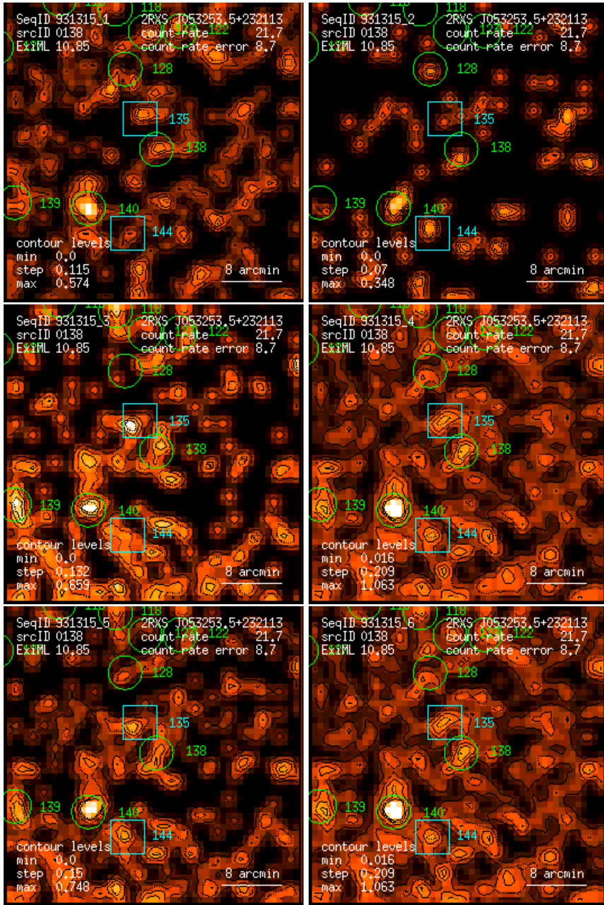
Figure 138: RASS 931315: detection 0138: band rate images, Gaussian filter: (1) PSPC channels 11 – 41, (2) 52 – 90, (3) 91 – 201, (4) 11 – 235, (5) 52 – 201, (6) 11 – 201. Broad band rates in counts/ks. Band rate contour levels in counts/ks/arcmin 2 .
