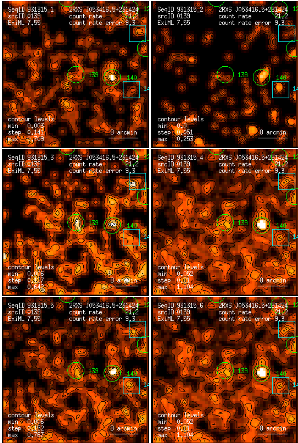
Figure 139: RASS 931315: detection 0139: band rate images, Gaussian filter: (1) PSPC channels 11 – 41, (2) 52 – 90, (3) 91 – 201, (4) 11 – 235, (5) 52 – 201, (6) 11 – 201. Broad band rates in counts/ks. Band rate contour levels in counts/ks/arcmin 2 .
