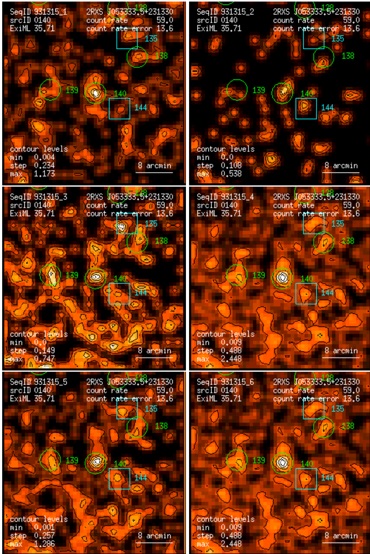
Figure 140: RASS 931315: detection 0140: band rate images, Gaussian filter: (1) PSPC channels 11 – 41, (2) 52 – 90, (3) 91 – 201, (4) 11 – 235, (5) 52 – 201, (6) 11 – 201. Broad band rates in counts/ks. Band rate contour levels in counts/ks/arcmin 2 .
