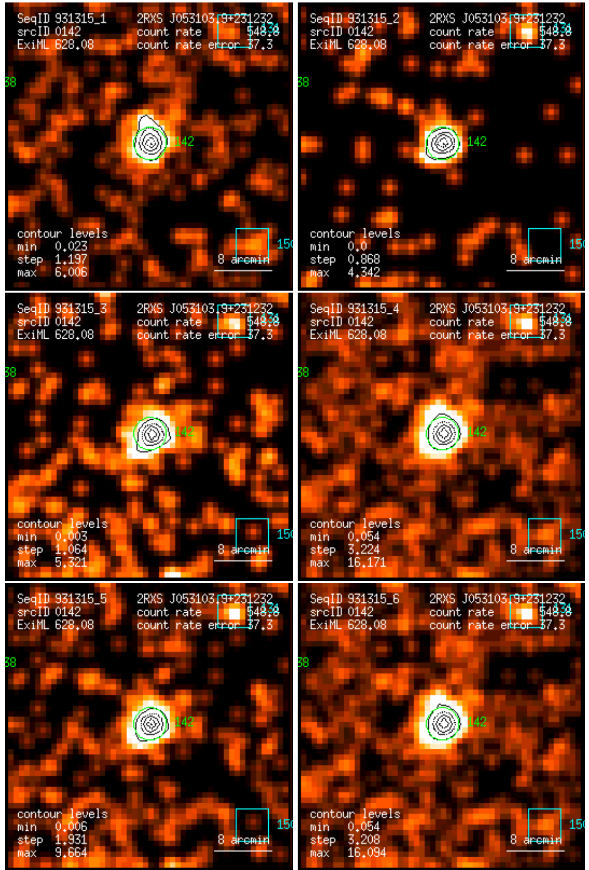
Figure 142: RASS 931315: detection 0142: band rate images, Gaussian filter: (1) PSPC channels 11 – 41, (2) 52 – 90, (3) 91 – 201, (4) 11 – 235, (5) 52 – 201, (6) 11 – 201. Broad band rates in counts/ks. Band rate contour levels in counts/ks/arcmin 2 .
