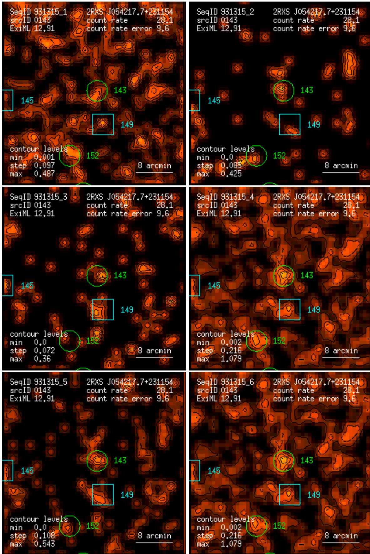
Figure 143: RASS 931315: detection 0143: band rate images, Gaussian filter: (1) PSPC channels 11 – 41, (2) 52 – 90, (3) 91 – 201, (4) 11 – 235, (5) 52 – 201, (6) 11 – 201. Broad band rates in counts/ks. Band rate contour levels in counts/ks/arcmin 2 .
