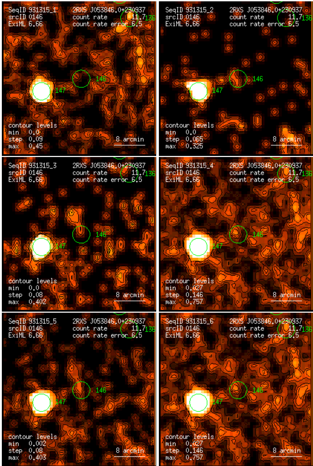
Figure 146: RASS 931315: detection 0146: band rate images, Gaussian filter: (1) PSPC channels 11 – 41, (2) 52 – 90, (3) 91 – 201, (4) 11 – 235, (5) 52 – 201, (6) 11 – 201. Broad band rates in counts/ks. Band rate contour levels in counts/ks/arcmin 2 .
