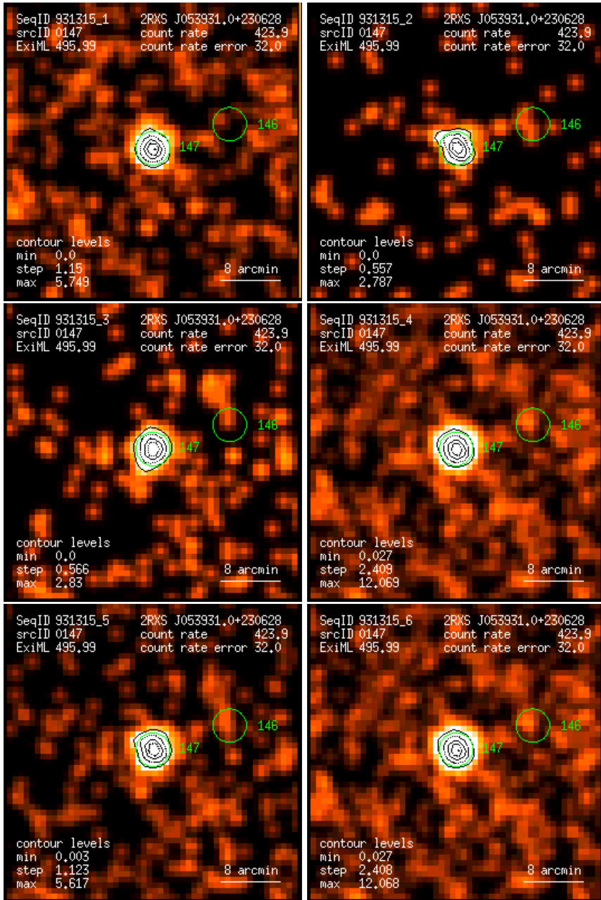
Figure 147: RASS 931315: detection 0147: band rate images, Gaussian filter: (1) PSPC channels 11 – 41, (2) 52 – 90, (3) 91 – 201, (4) 11 – 235, (5) 52 – 201, (6) 11 – 201. Broad band rates in counts/ks. Band rate contour levels in counts/ks/arcmin 2 .
