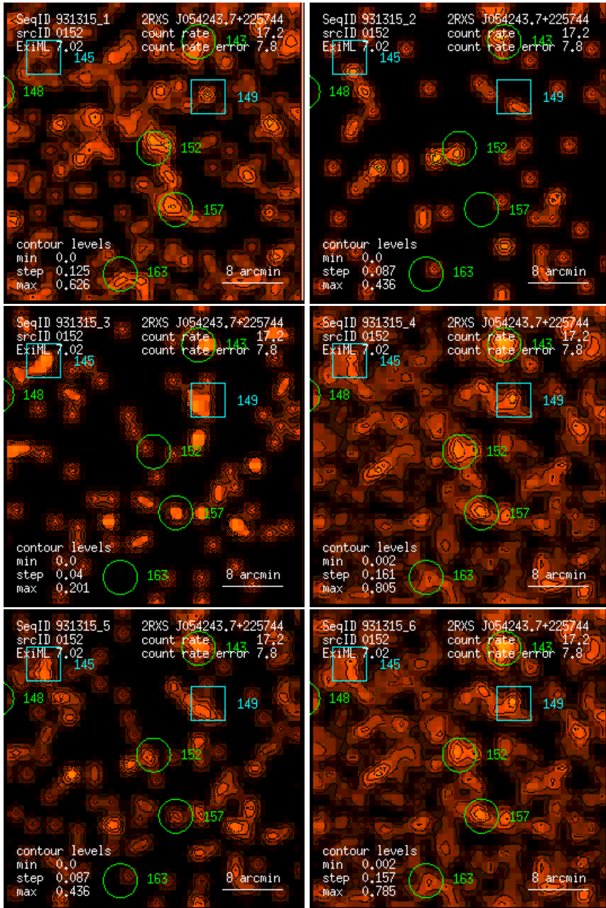
Figure 152: RASS 931315: detection 0152: band rate images, Gaussian filter: (1) PSPC channels 11 – 41, (2) 52 – 90, (3) 91 – 201, (4) 11 – 235, (5) 52 – 201, (6) 11 – 201. Broad band rates in counts/ks. Band rate contour levels in counts/ks/arcmin 2 .
