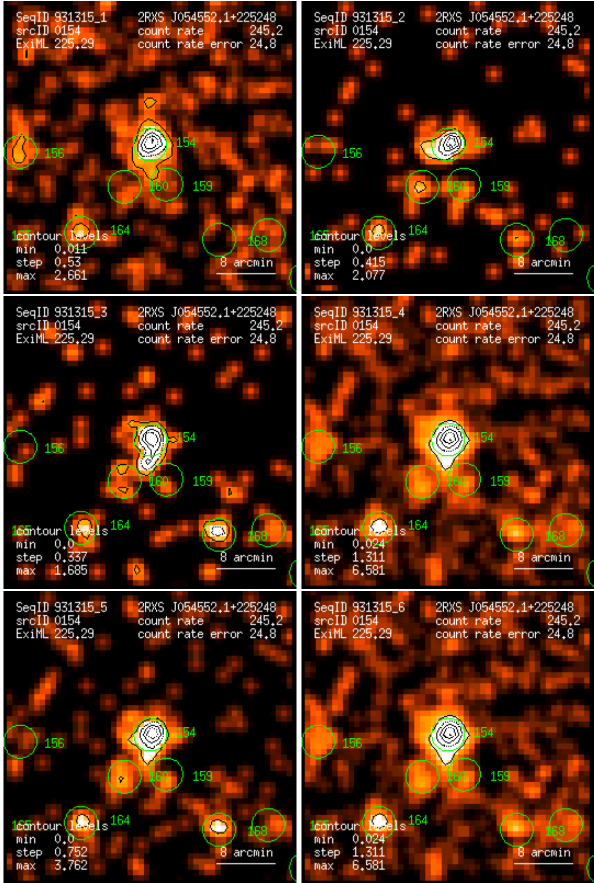
Figure 154: RASS 931315: detection 0154: band rate images, Gaussian filter: (1) PSPC channels 11 – 41, (2) 52 – 90, (3) 91 – 201, (4) 11 – 235, (5) 52 – 201, (6) 11 – 201. Broad band rates in counts/ks. Band rate contour levels in counts/ks/arcmin 2 .
