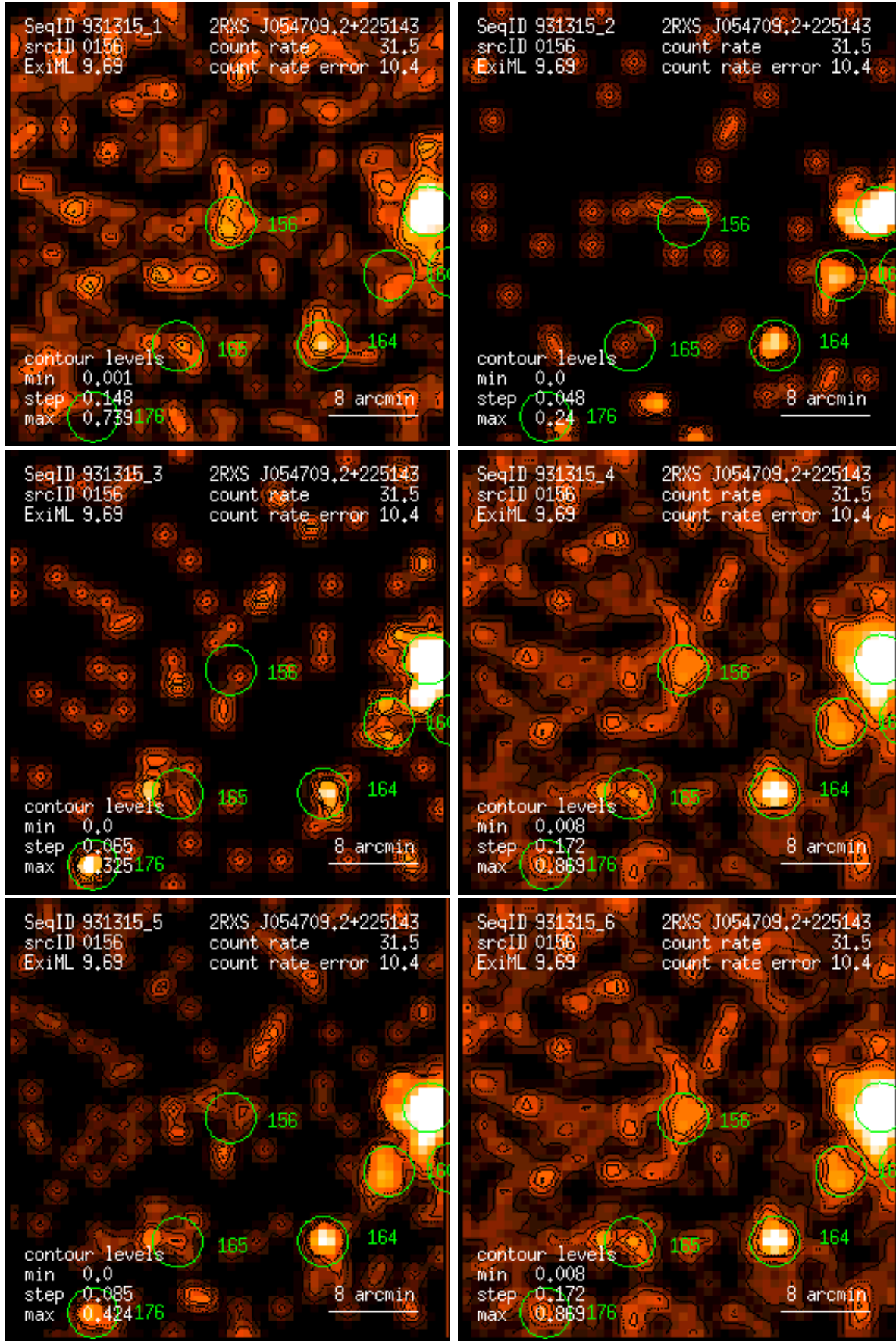
Figure 156: RASS 931315: detection 0156: band rate images, Gaussian filter: (1) PSPC channels 11 – 41, (2) 52 – 90, (3) 91 – 201, (4) 11 – 235, (5) 52 – 201, (6) 11 – 201. Broad band rates in counts/ks. Band rate contour levels in counts/ks/arcmin 2 .
