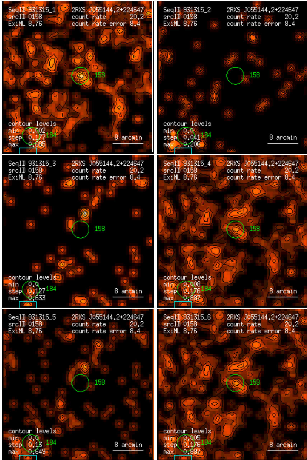
Figure 158: RASS 931315: detection 0158: band rate images, Gaussian filter: (1) PSPC channels 11 – 41, (2) 52 – 90, (3) 91 – 201, (4) 11 – 235, (5) 52 – 201, (6) 11 – 201. Broad band rates in counts/ks. Band rate contour levels in counts/ks/arcmin 2 .
