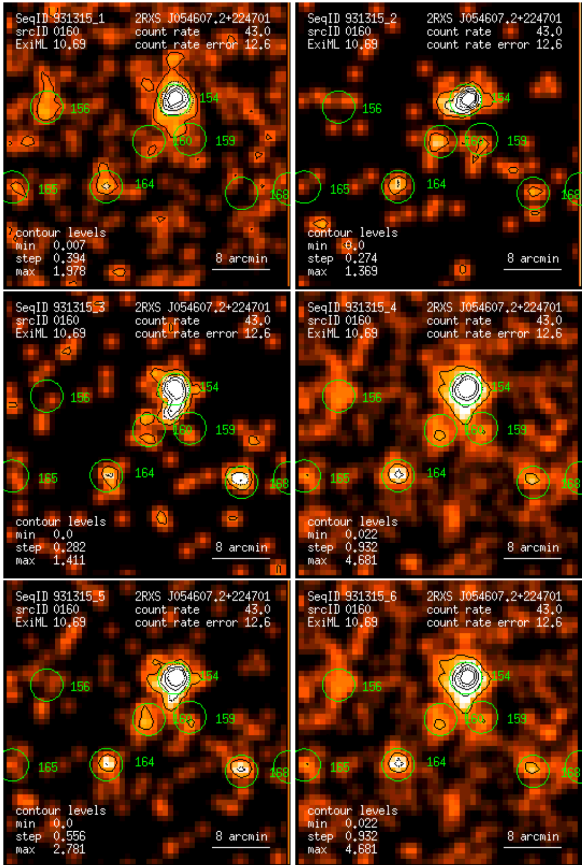
Figure 160: RASS 931315: detection 0160: band rate images, Gaussian filter: (1) PSPC channels 11 – 41, (2) 52 – 90, (3) 91 – 201, (4) 11 – 235, (5) 52 – 201, (6) 11 – 201. Broad band rates in counts/ks. Band rate contour levels in counts/ks/arcmin 2 .
