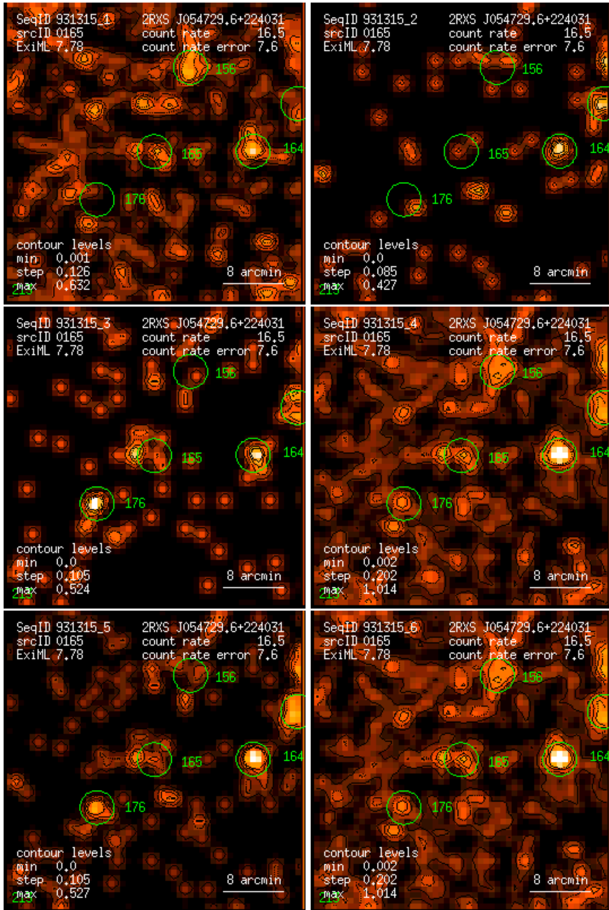
Figure 165: RASS 931315: detection 0165: band rate images, Gaussian filter: (1) PSPC channels 11 – 41, (2) 52 – 90, (3) 91 – 201, (4) 11 – 235, (5) 52 – 201, (6) 11 – 201. Broad band rates in counts/ks. Band rate contour levels in counts/ks/arcmin 2 .
