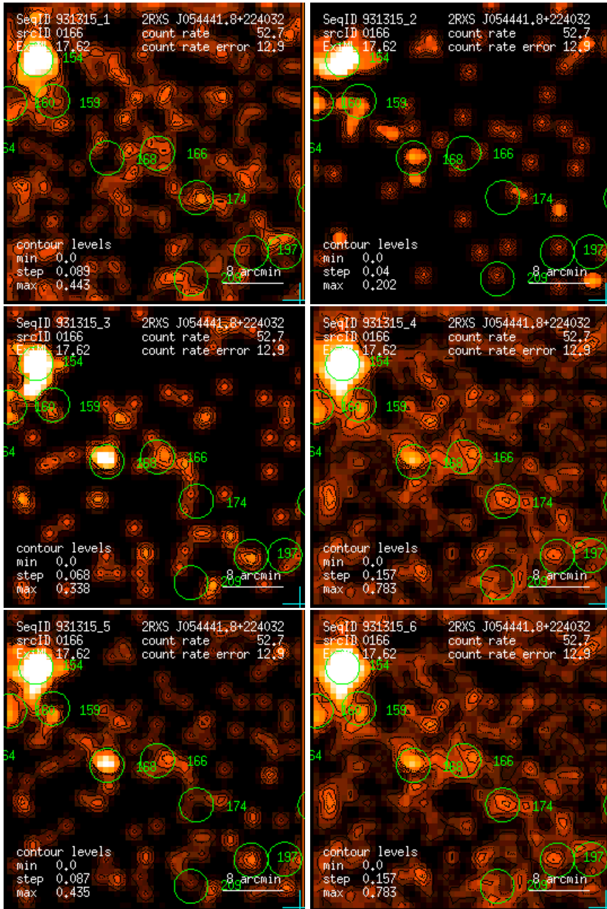
Figure 166: RASS 931315: detection 0166: band rate images, Gaussian filter: (1) PSPC channels 11 – 41, (2) 52 – 90, (3) 91 – 201, (4) 11 – 235, (5) 52 – 201, (6) 11 – 201. Broad band rates in counts/ks. Band rate contour levels in counts/ks/arcmin 2 .
