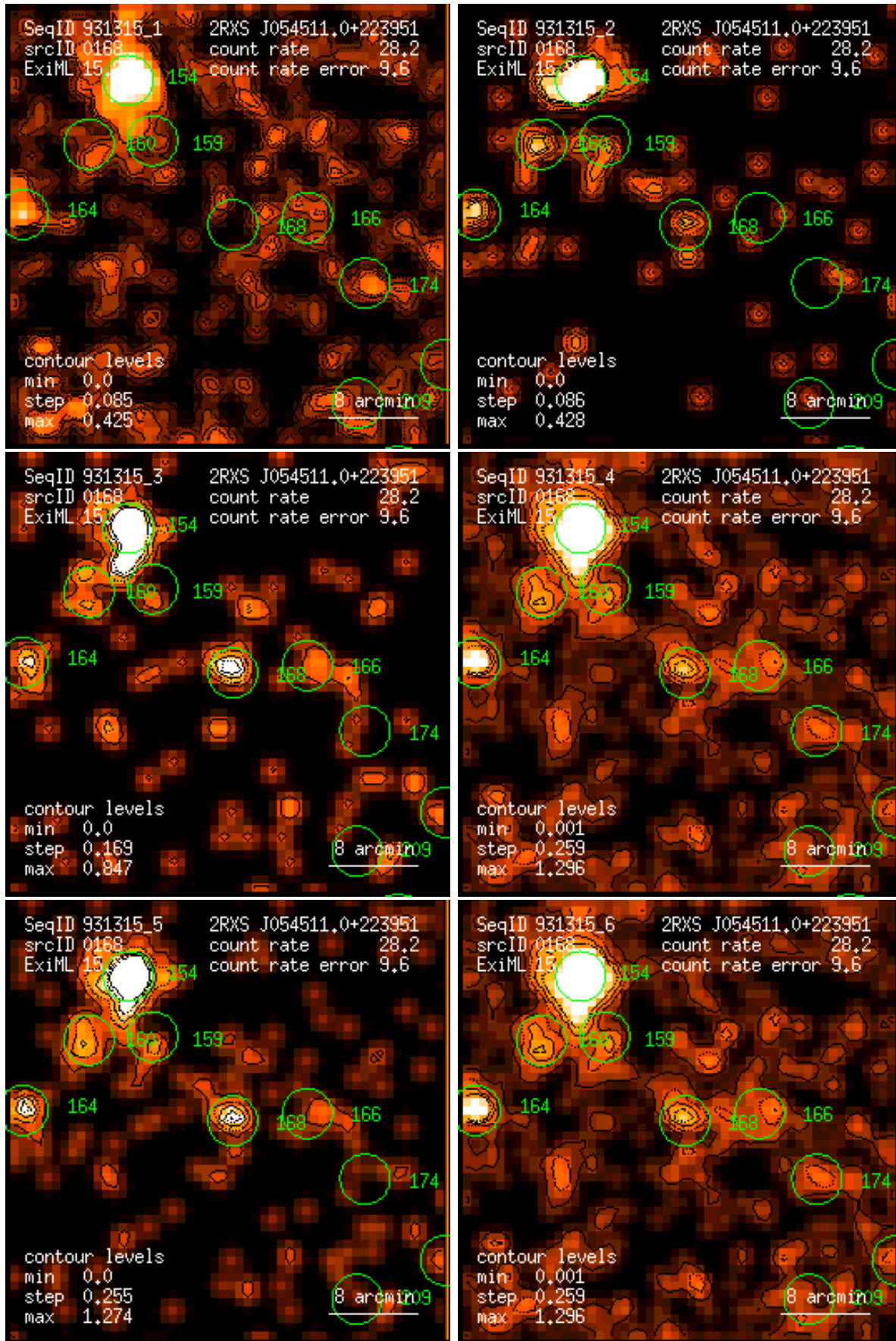
Figure 168: RASS 931315: detection 0168: band rate images, Gaussian filter: (1) PSPC channels 11 – 41, (2) 52 – 90, (3) 91 – 201, (4) 11 – 235, (5) 52 – 201, (6) 11 – 201. Broad band rates in counts/ks. Band rate contour levels in counts/ks/arcmin 2 .
