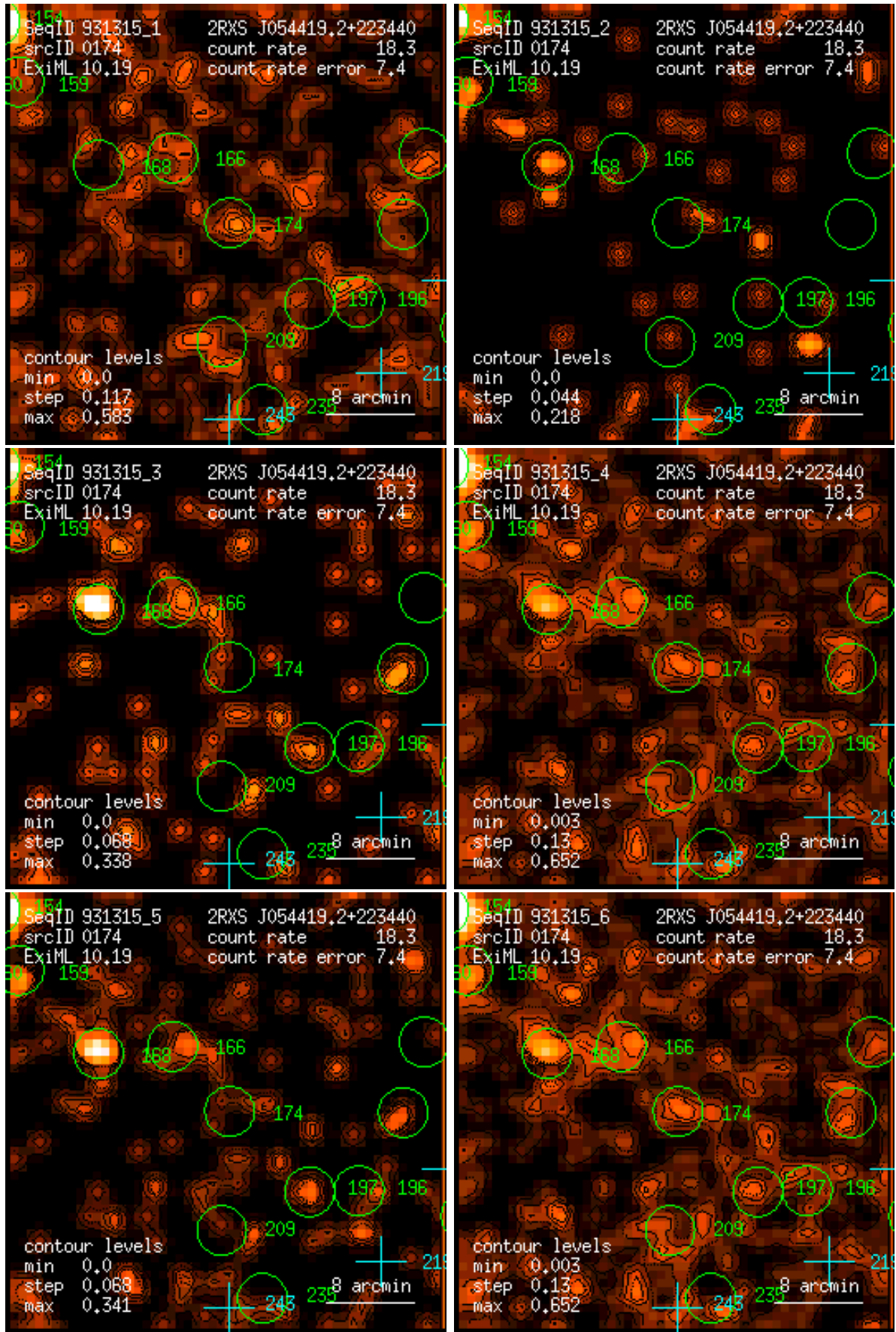
Figure 174: RASS 931315: detection 0174: band rate images, Gaussian filter: (1) PSPC channels 11 – 41, (2) 52 – 90, (3) 91 – 201, (4) 11 – 235, (5) 52 – 201, (6) 11 – 201. Broad band rates in counts/ks. Band rate contour levels in counts/ks/arcmin 2 .
