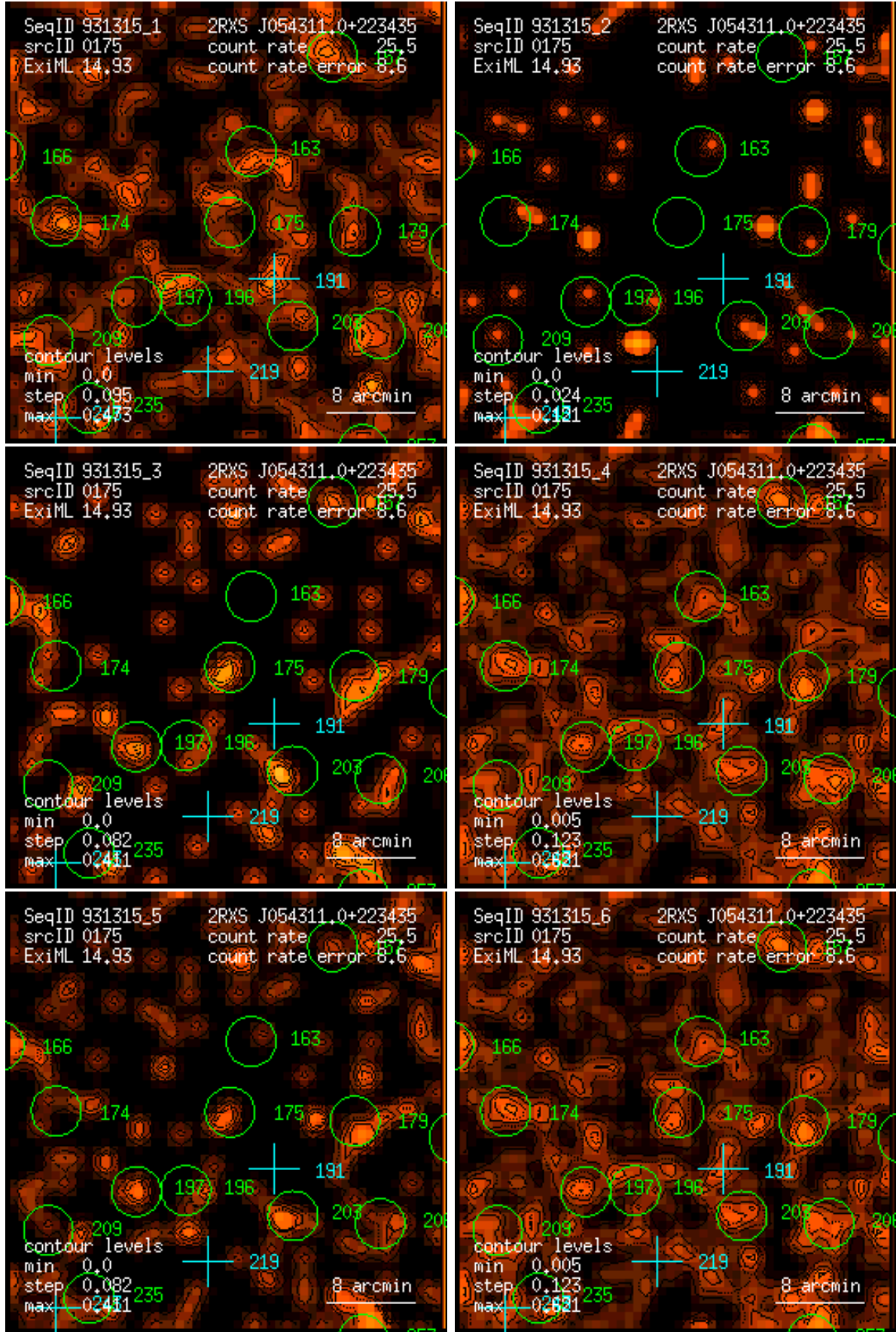
Figure 175: RASS 931315: detection 0175: band rate images, Gaussian filter: (1) PSPC channels 11 – 41, (2) 52 – 90, (3) 91 – 201, (4) 11 – 235, (5) 52 – 201, (6) 11 – 201. Broad band rates in counts/ks. Band rate contour levels in counts/ks/arcmin 2 .
