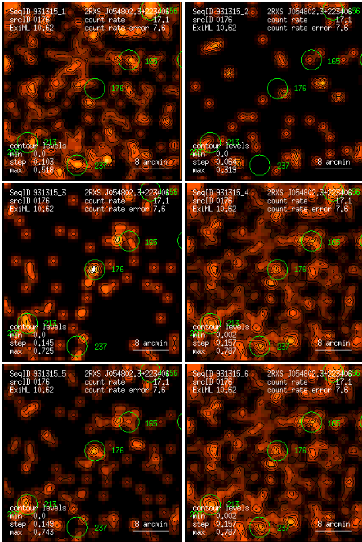
Figure 176: RASS 931315: detection 0176: band rate images, Gaussian filter: (1) PSPC channels 11 – 41, (2) 52 – 90, (3) 91 – 201, (4) 11 – 235, (5) 52 – 201, (6) 11 – 201. Broad band rates in counts/ks. Band rate contour levels in counts/ks/arcmin 2 .
