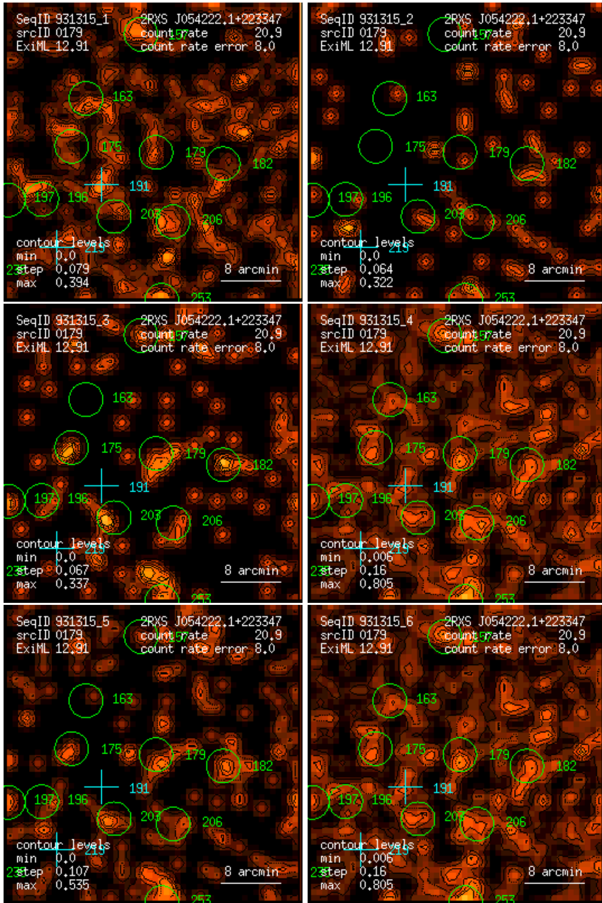
Figure 179: RASS 931315: detection 0179: band rate images, Gaussian filter: (1) PSPC channels 11 – 41, (2) 52 – 90, (3) 91 – 201, (4) 11 – 235, (5) 52 – 201, (6) 11 – 201. Broad band rates in counts/ks. Band rate contour levels in counts/ks/arcmin 2 .
