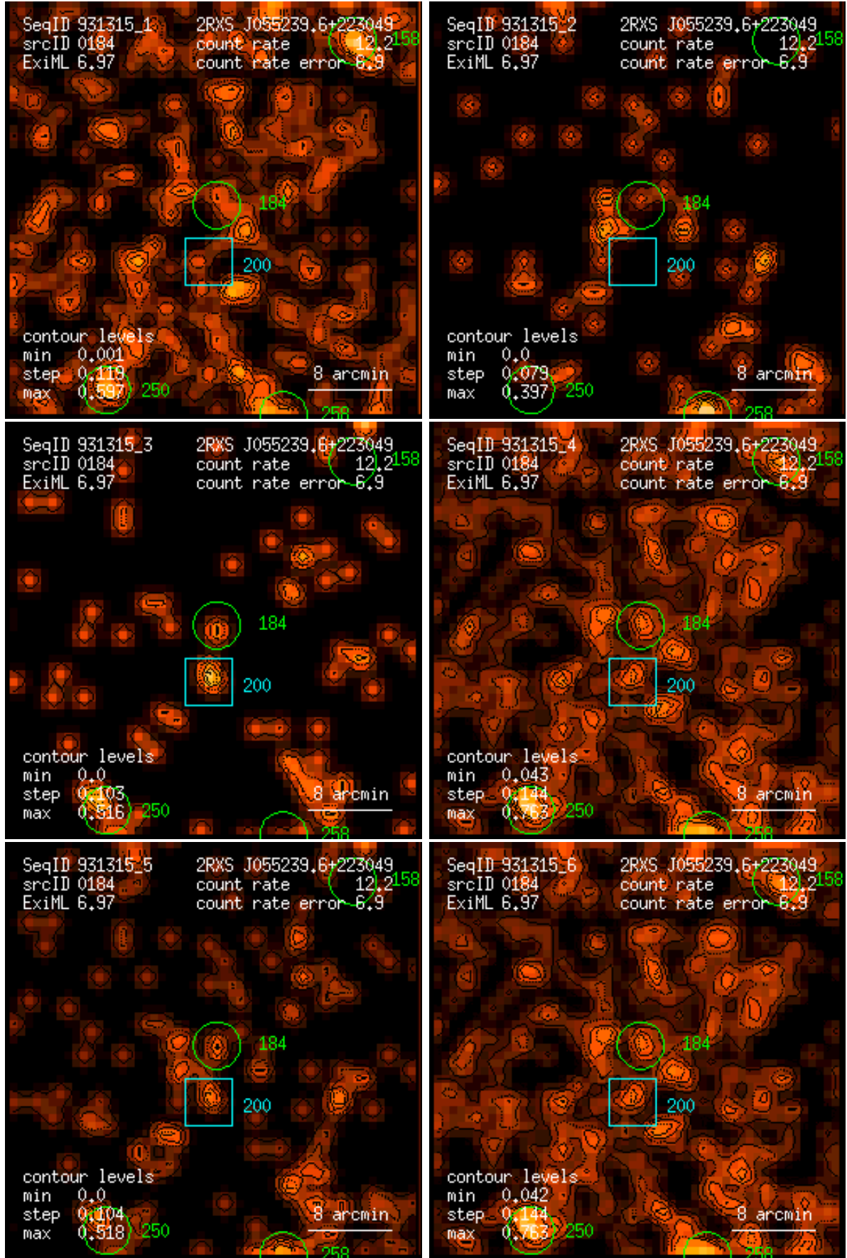
Figure 184: RASS 931315: detection 0184: band rate images, Gaussian filter: (1) PSPC channels 11 – 41, (2) 52 – 90, (3) 91 – 201, (4) 11 – 235, (5) 52 – 201, (6) 11 – 201. Broad band rates in counts/ks. Band rate contour levels in counts/ks/arcmin 2 .
