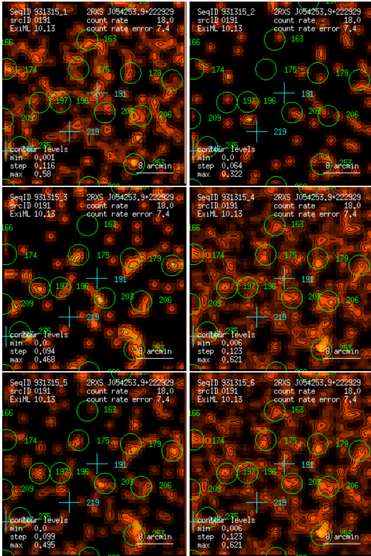
Figure 191: RASS 931315: detection 0191: band rate images, Gaussian filter: (1) PSPC channels 11 – 41, (2) 52 – 90, (3) 91 – 201, (4) 11 – 235, (5) 52 – 201, (6) 11 – 201. Broad band rates in counts/ks. Band rate contour levels in counts/ks/arcmin 2 .
