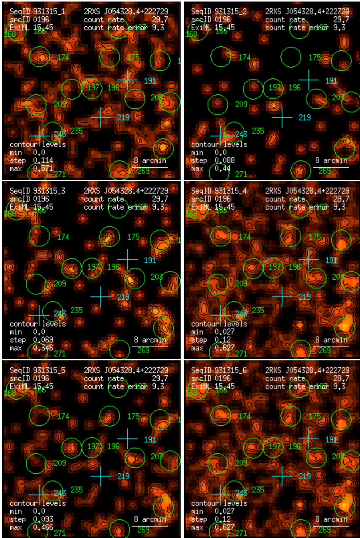
Figure 196: RASS 931315: detection 0196: band rate images, Gaussian filter: (1) PSPC channels 11 – 41, (2) 52 – 90, (3) 91 – 201, (4) 11 – 235, (5) 52 – 201, (6) 11 – 201. Broad band rates in counts/ks. Band rate contour levels in counts/ks/arcmin 2 .
