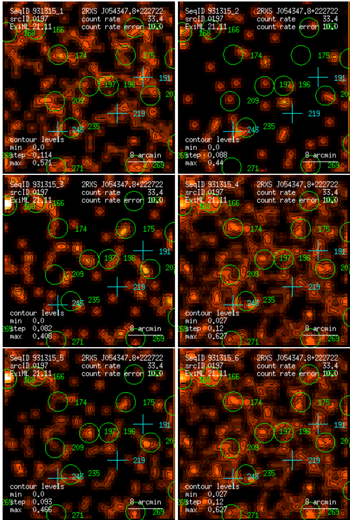
Figure 197: RASS 931315: detection 0197: band rate images, Gaussian filter: (1) PSPC channels 11 – 41, (2) 52 – 90, (3) 91 – 201, (4) 11 – 235, (5) 52 – 201, (6) 11 – 201. Broad band rates in counts/ks. Band rate contour levels in counts/ks/arcmin 2 .
