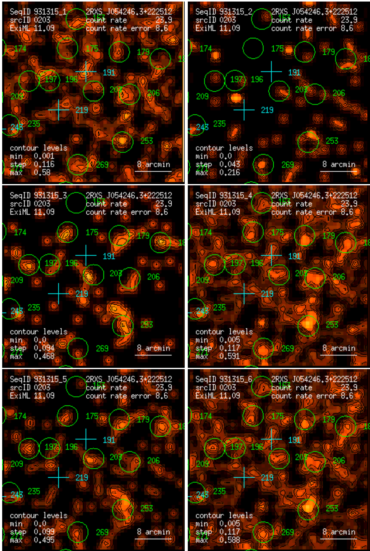
Figure 203: RASS 931315: detection 0203: band rate images, Gaussian filter: (1) PSPC channels 11 – 41, (2) 52 – 90, (3) 91 – 201, (4) 11 – 235, (5) 52 – 201, (6) 11 – 201. Broad band rates in counts/ks. Band rate contour levels in counts/ks/arcmin 2 .
