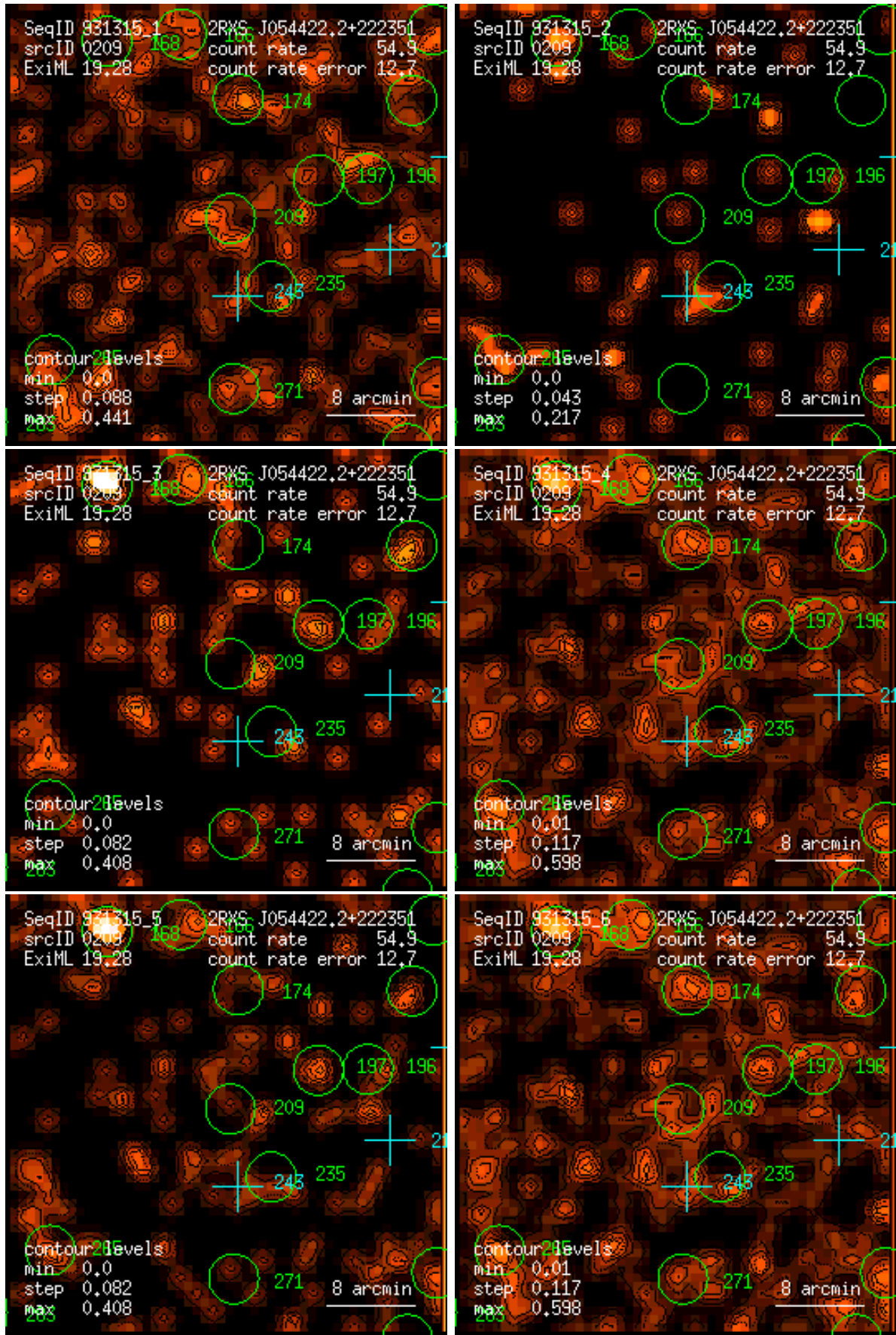
Figure 209: RASS 931315: detection 0209: band rate images, Gaussian filter: (1) PSPC channels 11 – 41, (2) 52 – 90, (3) 91 – 201, (4) 11 – 235, (5) 52 – 201, (6) 11 – 201. Broad band rates in counts/ks. Band rate contour levels in counts/ks/arcmin 2 .
