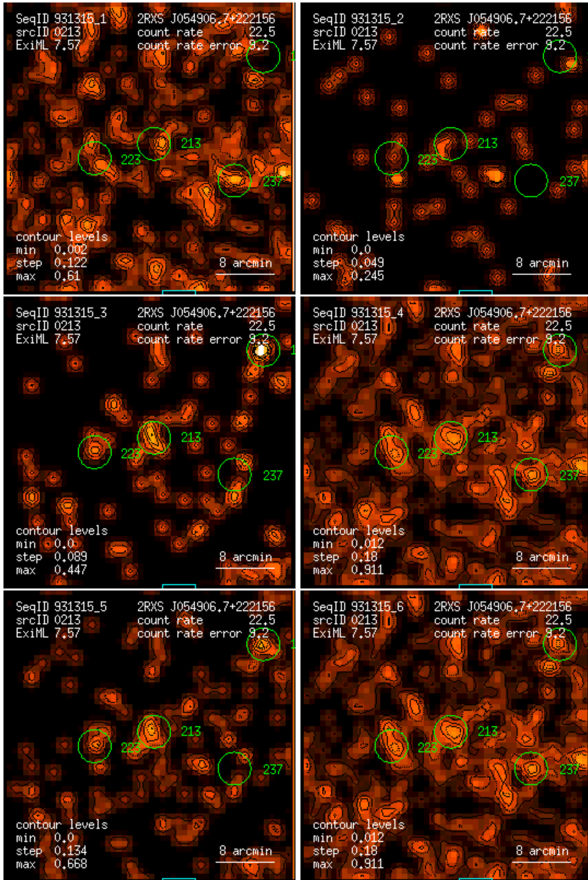
Figure 213: RASS 931315: detection 0213: band rate images, Gaussian filter: (1) PSPC channels 11 – 41, (2) 52 – 90, (3) 91 – 201, (4) 11 – 235, (5) 52 – 201, (6) 11 – 201. Broad band rates in counts/ks. Band rate contour levels in counts/ks/arcmin 2 .
