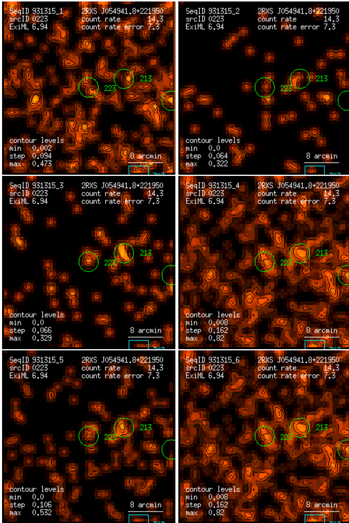
Figure 223: RASS 931315: detection 0223: band rate images, Gaussian filter: (1) PSPC channels 11 – 41, (2) 52 – 90, (3) 91 – 201, (4) 11 – 235, (5) 52 – 201, (6) 11 – 201. Broad band rates in counts/ks. Band rate contour levels in counts/ks/arcmin 2 .
