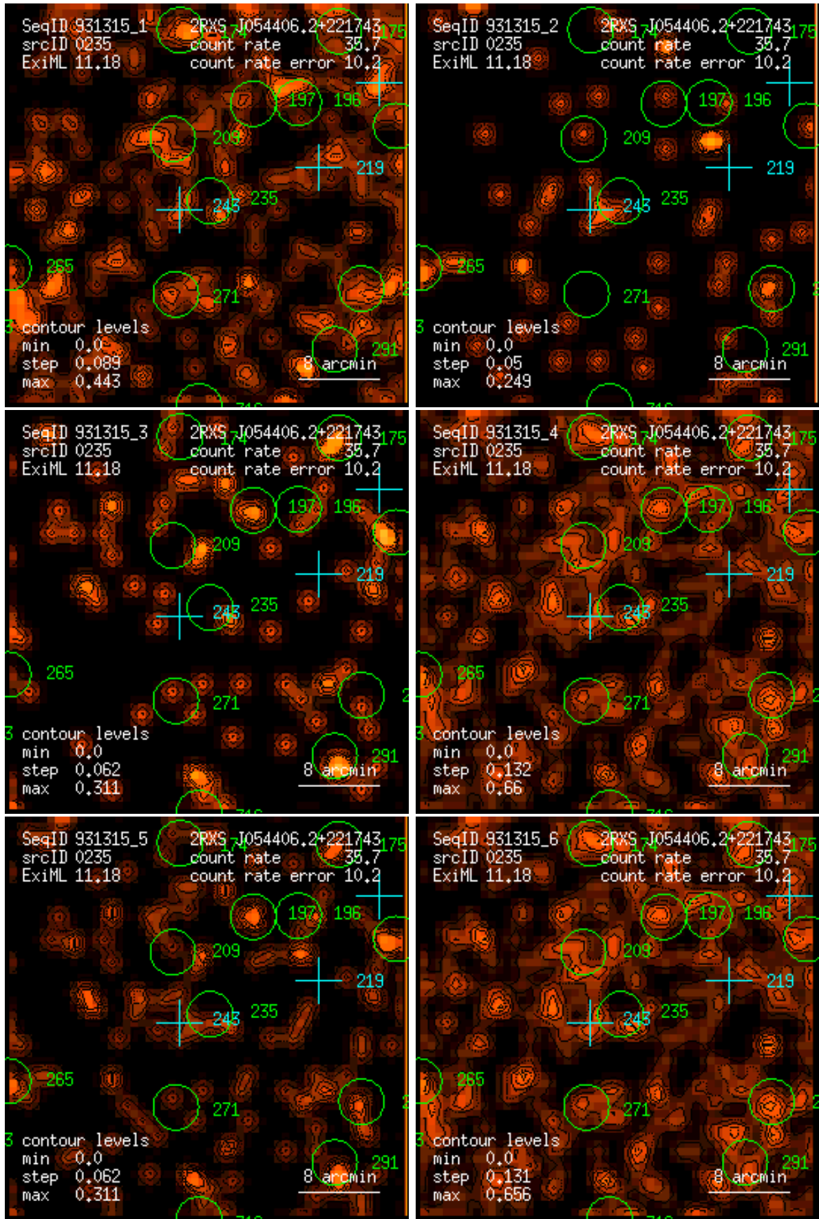
Figure 235: RASS 931315: detection 0235: band rate images, Gaussian filter: (1) PSPC channels 11 – 41, (2) 52 – 90, (3) 91 – 201, (4) 11 – 235, (5) 52 – 201, (6) 11 – 201. Broad band rates in counts/ks. Band rate contour levels in counts/ks/arcmin 2 .
