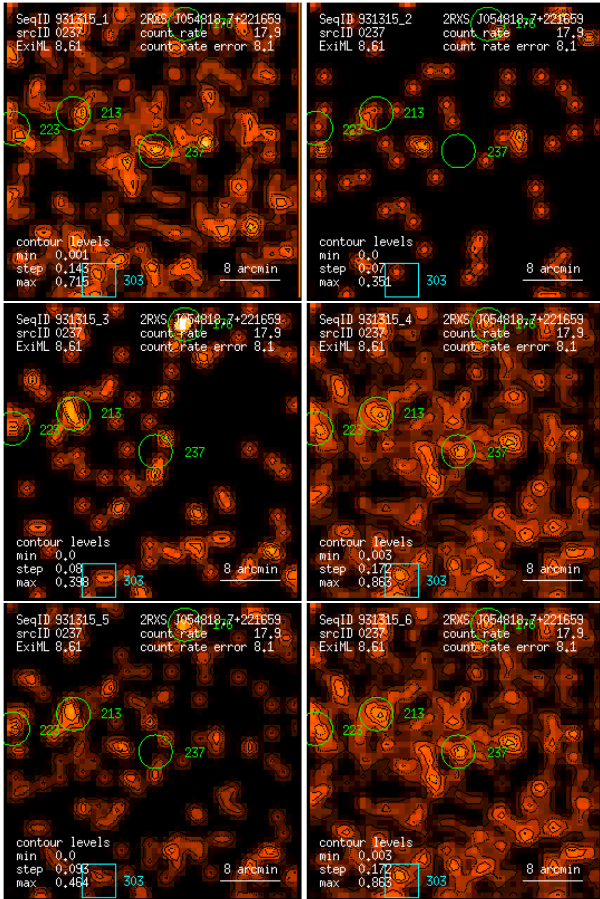
Figure 237: RASS 931315: detection 0237: band rate images, Gaussian filter: (1) PSPC channels 11 – 41, (2) 52 – 90, (3) 91 – 201, (4) 11 – 235, (5) 52 – 201, (6) 11 – 201. Broad band rates in counts/ks. Band rate contour levels in counts/ks/arcmin 2 .
