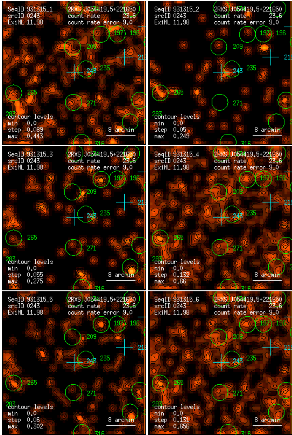
Figure 243: RASS 931315: detection 0243: band rate images, Gaussian filter: (1) PSPC channels 11 – 41, (2) 52 – 90, (3) 91 – 201, (4) 11 – 235, (5) 52 – 201, (6) 11 – 201. Broad band rates in counts/ks. Band rate contour levels in counts/ks/arcmin 2 .
