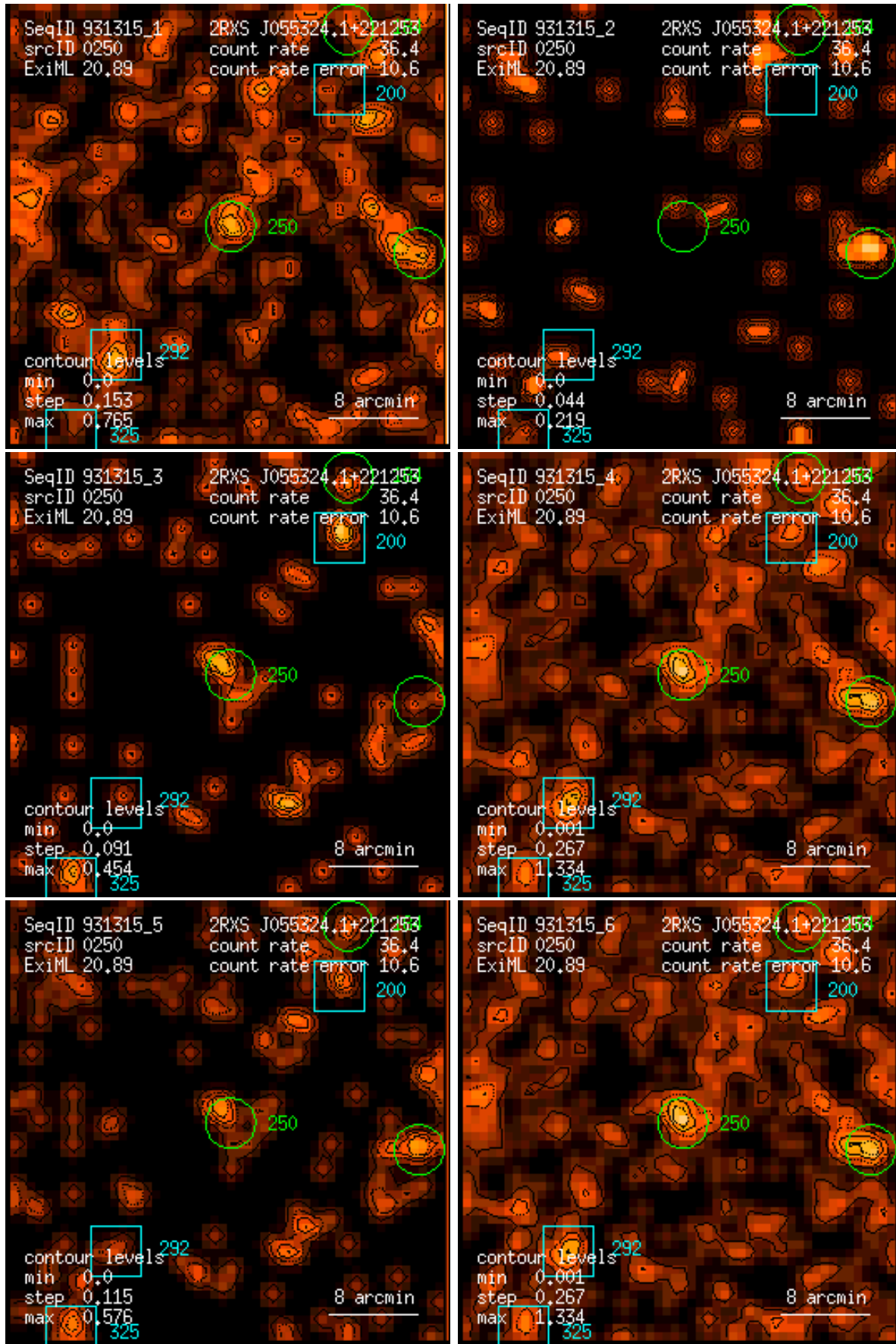
Figure 250: RASS 931315: detection 0250: band rate images, Gaussian filter: (1) PSPC channels 11 – 41, (2) 52 – 90, (3) 91 – 201, (4) 11 – 235, (5) 52 – 201, (6) 11 – 201. Broad band rates in counts/ks. Band rate contour levels in counts/ks/arcmin 2 .
