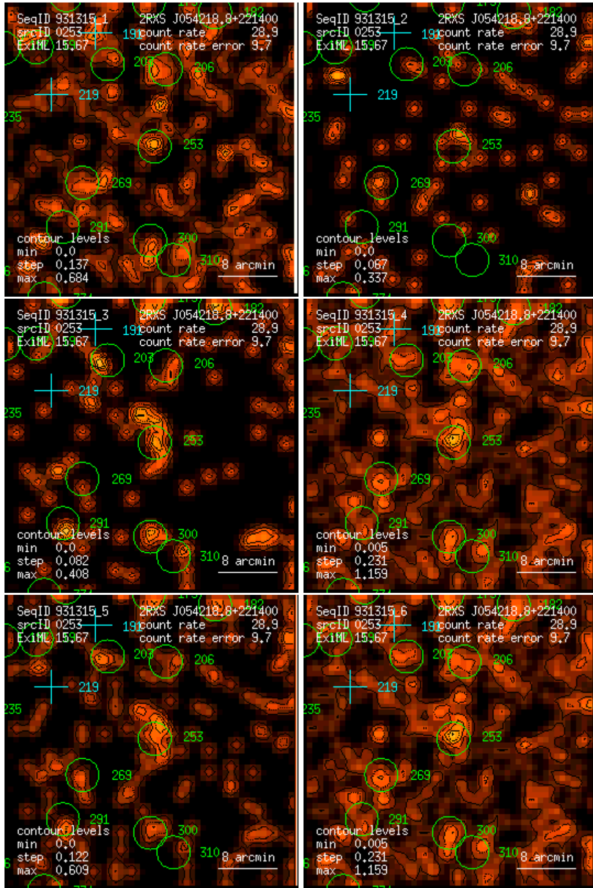
Figure 253: RASS 931315: detection 0253: band rate images, Gaussian filter: (1) PSPC channels 11 – 41, (2) 52 – 90, (3) 91 – 201, (4) 11 – 235, (5) 52 – 201, (6) 11 – 201. Broad band rates in counts/ks. Band rate contour levels in counts/ks/arcmin 2 .
