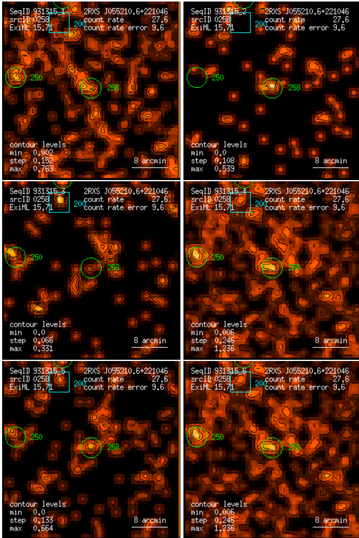
Figure 258: RASS 931315: detection 0258: band rate images, Gaussian filter: (1) PSPC channels 11 – 41, (2) 52 – 90, (3) 91 – 201, (4) 11 – 235, (5) 52 – 201, (6) 11 – 201. Broad band rates in counts/ks. Band rate contour levels in counts/ks/arcmin 2 .
