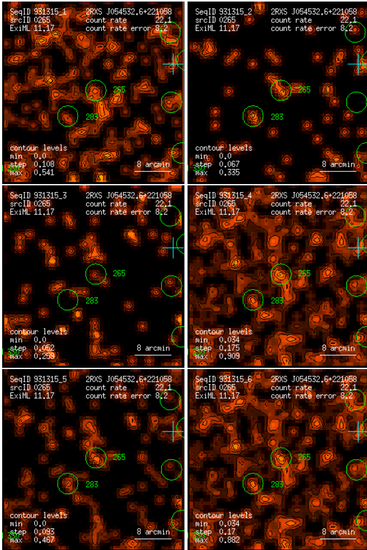
Figure 265: RASS 931315: detection 0265: band rate images, Gaussian filter: (1) PSPC channels 11 – 41, (2) 52 – 90, (3) 91 – 201, (4) 11 – 235, (5) 52 – 201, (6) 11 – 201. Broad band rates in counts/ks. Band rate contour levels in counts/ks/arcmin 2 .
