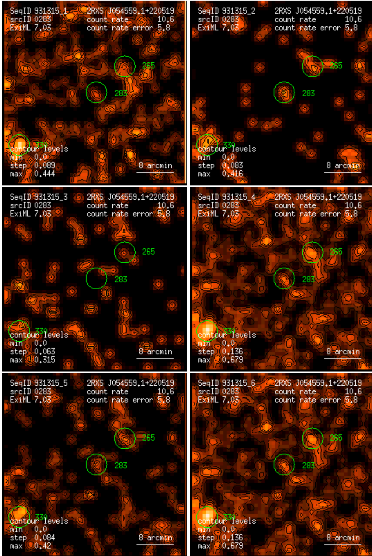
Figure 283: RASS 931315: detection 0283: band rate images, Gaussian filter: (1) PSPC channels 11 – 41, (2) 52 – 90, (3) 91 – 201, (4) 11 – 235, (5) 52 – 201, (6) 11 – 201. Broad band rates in counts/ks. Band rate contour levels in counts/ks/arcmin 2 .
