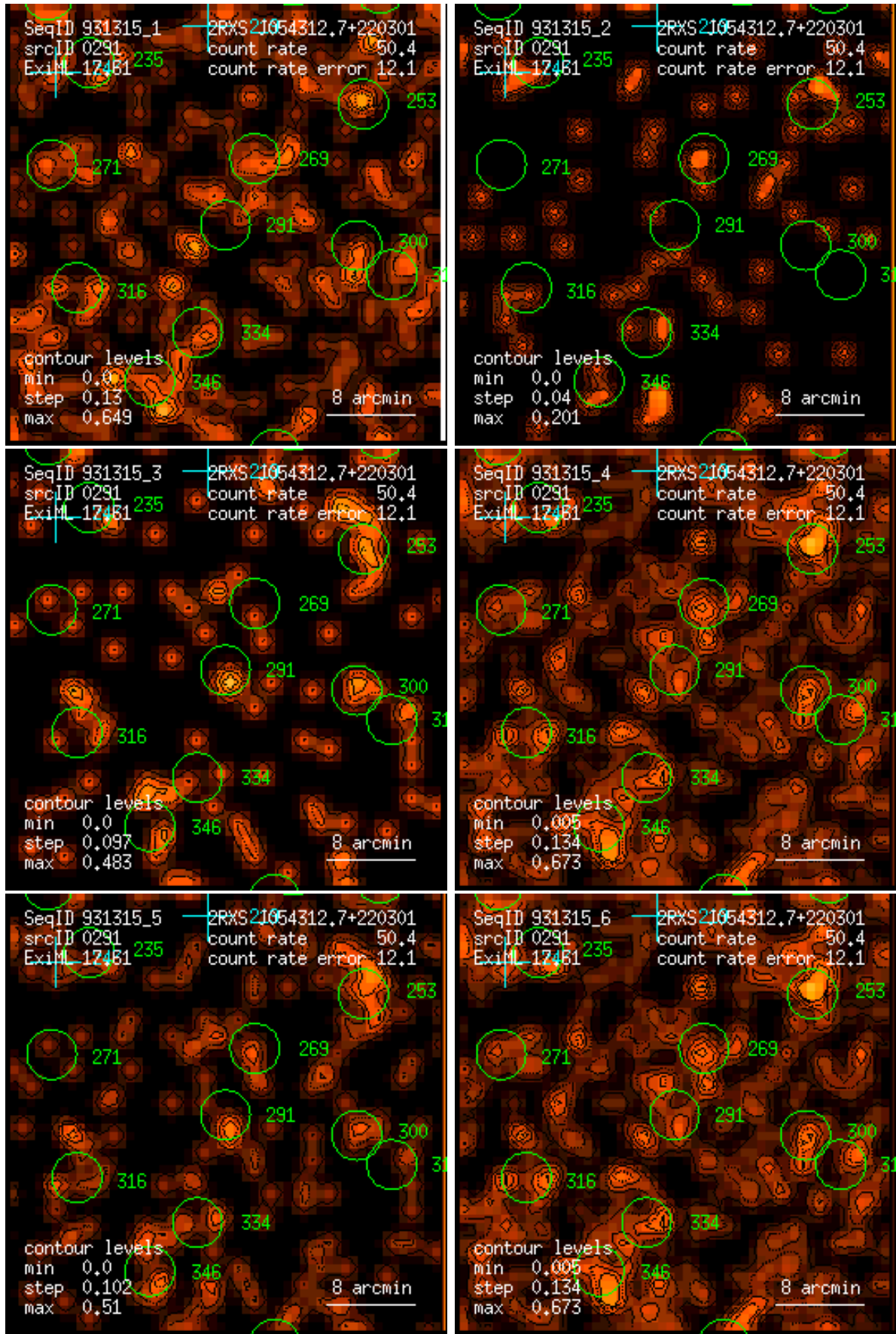
Figure 291: RASS 931315: detection 0291: band rate images, Gaussian filter: (1) PSPC channels 11 – 41, (2) 52 – 90, (3) 91 – 201, (4) 11 – 235, (5) 52 – 201, (6) 11 – 201. Broad band rates in counts/ks. Band rate contour levels in counts/ks/arcmin 2 .
