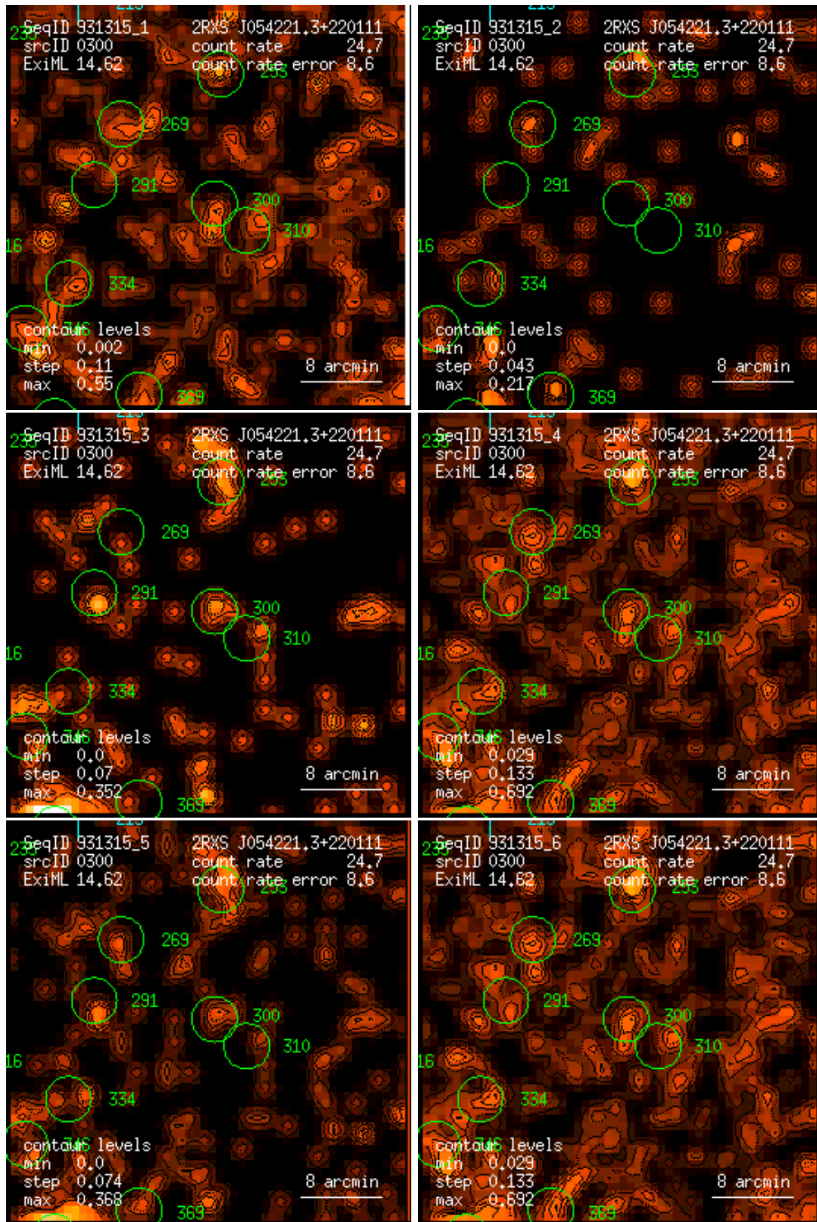
Figure 300: RASS 931315: detection 0300: band rate images, Gaussian filter: (1) PSPC channels 11 – 41, (2) 52 – 90, (3) 91 – 201, (4) 11 – 235, (5) 52 – 201, (6) 11 – 201. Broad band rates in counts/ks. Band rate contour levels in counts/ks/arcmin 2 .
