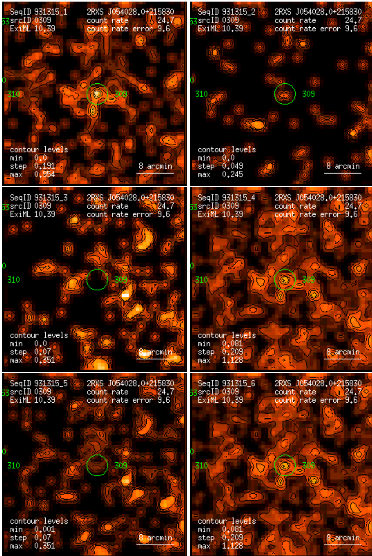
Figure 309: RASS 931315: detection 0309: band rate images, Gaussian filter: (1) PSPC channels 11 – 41, (2) 52 – 90, (3) 91 – 201, (4) 11 – 235, (5) 52 – 201, (6) 11 – 201. Broad band rates in counts/ks. Band rate contour levels in counts/ks/arcmin 2 .
