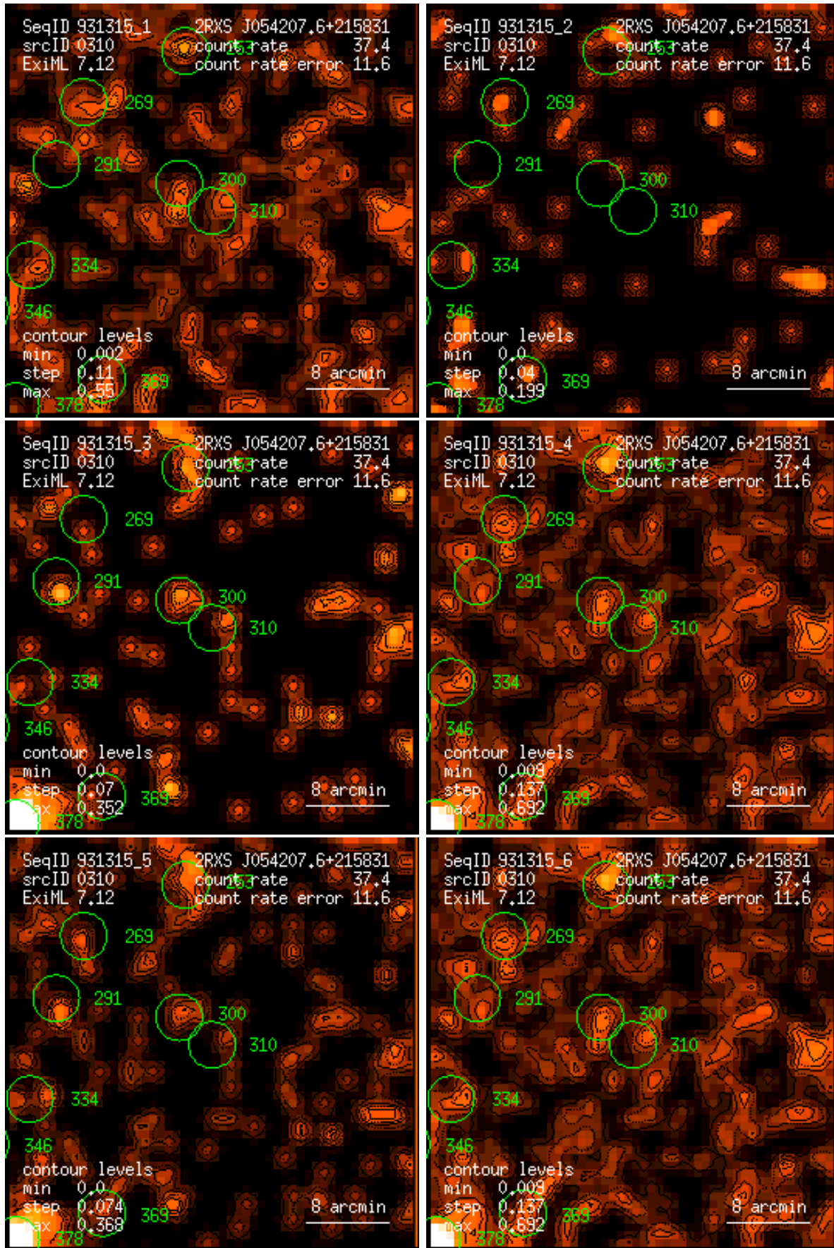
Figure 310: RASS 931315: detection 0310: band rate images, Gaussian filter: (1) PSPC channels 11 – 41, (2) 52 – 90, (3) 91 – 201, (4) 11 – 235, (5) 52 – 201, (6) 11 – 201. Broad band rates in counts/ks. Band rate contour levels in counts/ks/arcmin 2 .
