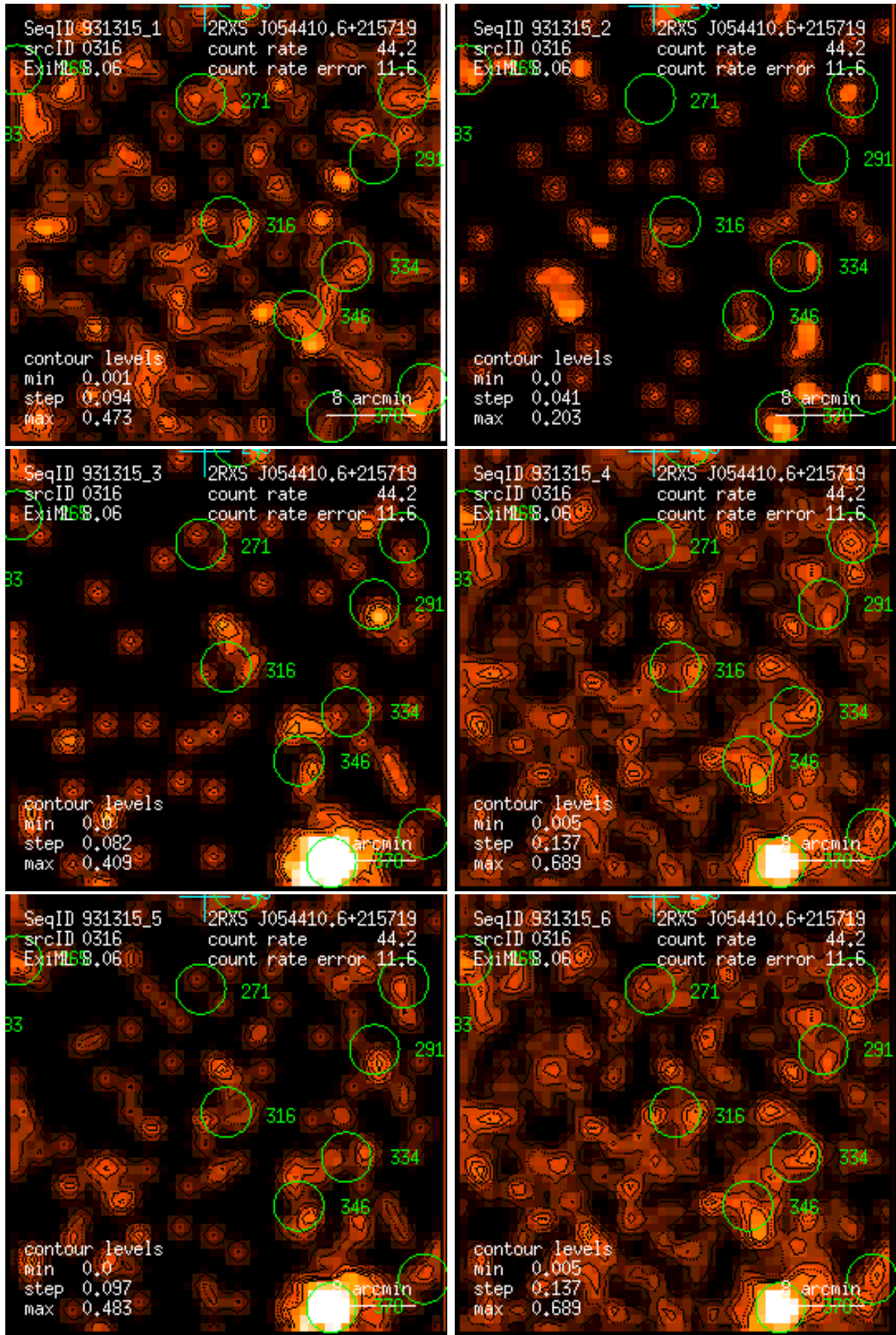
Figure 316: RASS 931315: detection 0316: band rate images, Gaussian filter: (1) PSPC channels 11 – 41, (2) 52 – 90, (3) 91 – 201, (4) 11 – 235, (5) 52 – 201, (6) 11 – 201. Broad band rates in counts/ks. Band rate contour levels in counts/ks/arcmin 2 .
