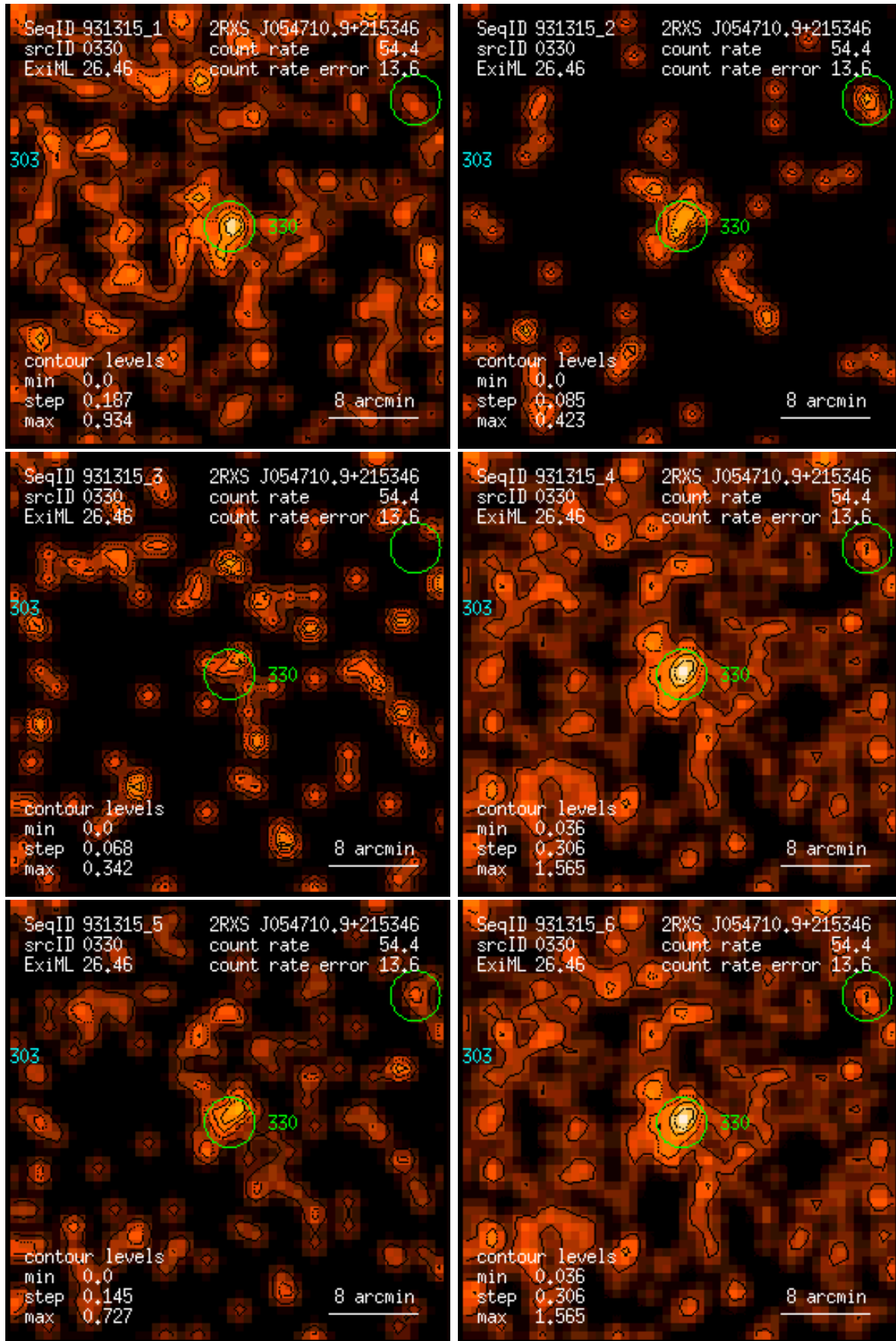
Figure 330: RASS 931315: detection 0330: band rate images, Gaussian filter: (1) PSPC channels 11 – 41, (2) 52 – 90, (3) 91 – 201, (4) 11 – 235, (5) 52 – 201, (6) 11 – 201. Broad band rates in counts/ks. Band rate contour levels in counts/ks/arcmin 2 .
