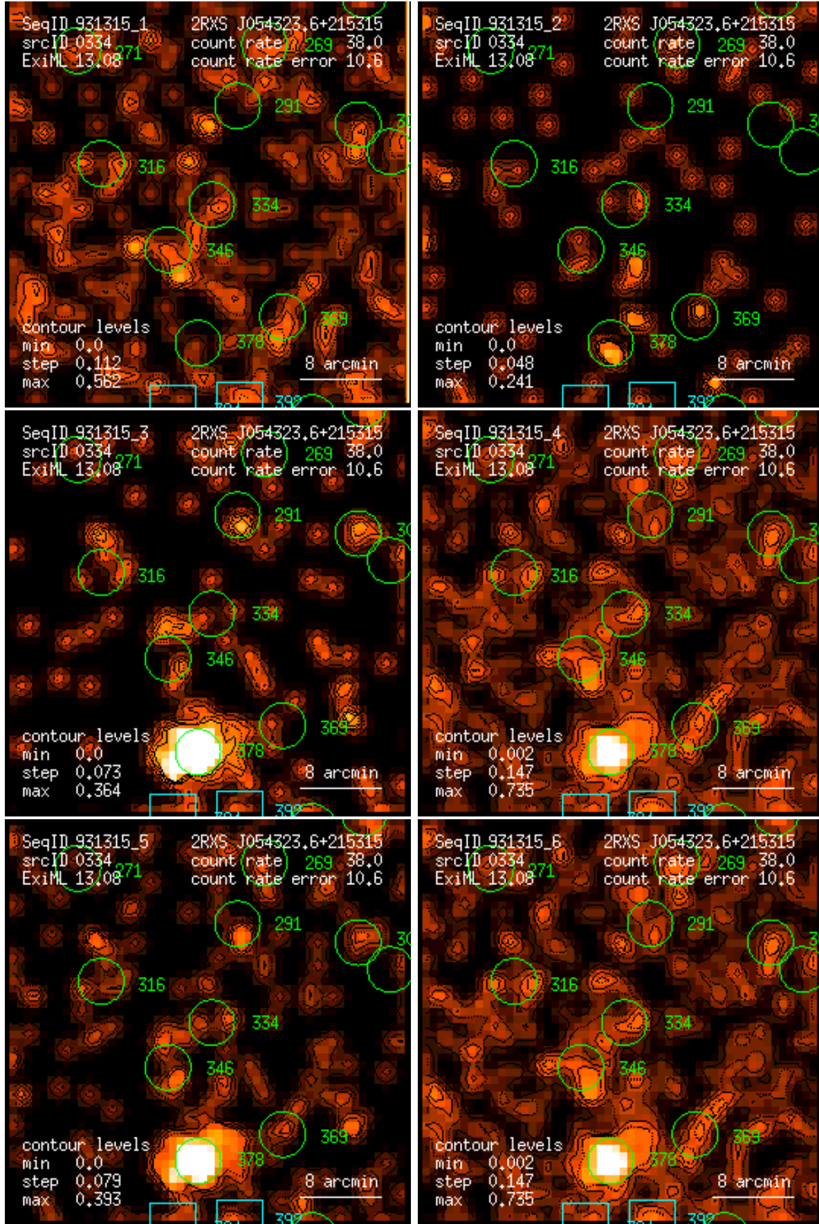
Figure 334: RASS 931315: detection 0334: band rate images, Gaussian filter: (1) PSPC channels 11 – 41, (2) 52 – 90, (3) 91 – 201, (4) 11 – 235, (5) 52 – 201, (6) 11 – 201. Broad band rates in counts/ks. Band rate contour levels in counts/ks/arcmin 2 .
