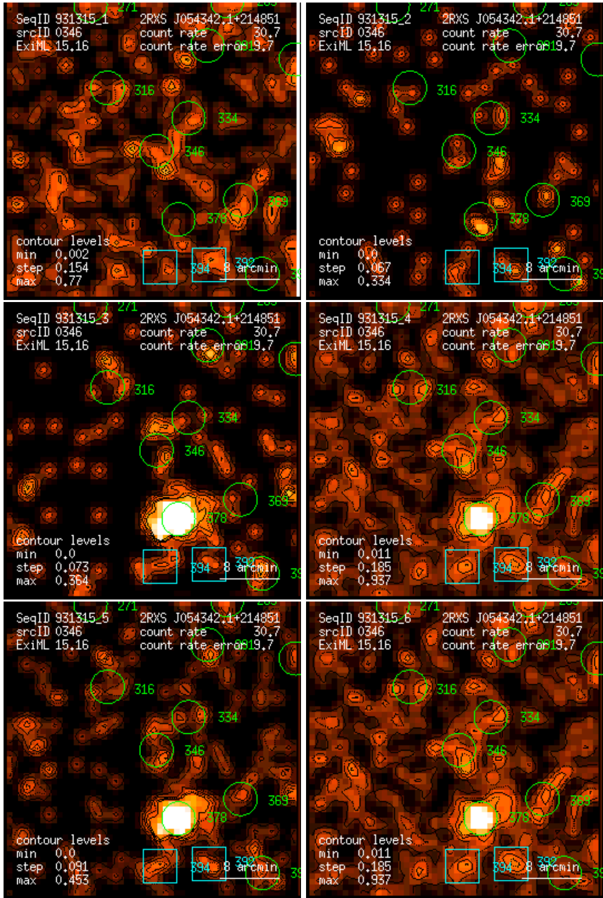
Figure 346: RASS 931315: detection 0346: band rate images, Gaussian filter: (1) PSPC channels 11 – 41, (2) 52 – 90, (3) 91 – 201, (4) 11 – 235, (5) 52 – 201, (6) 11 – 201. Broad band rates in counts/ks. Band rate contour levels in counts/ks/arcmin 2 .
