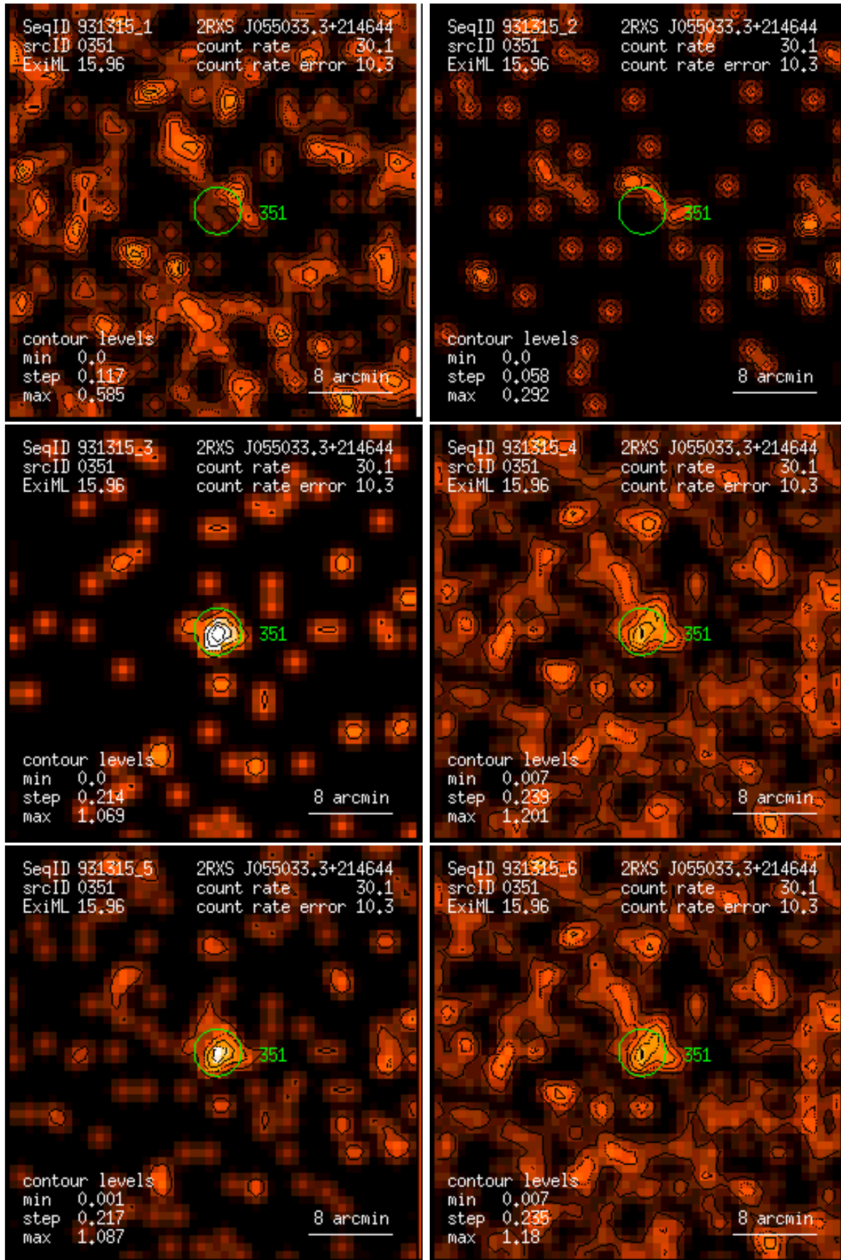
Figure 351: RASS 931315: detection 0351: band rate images, Gaussian filter: (1) PSPC channels 11 – 41, (2) 52 – 90, (3) 91 – 201, (4) 11 – 235, (5) 52 – 201, (6) 11 – 201. Broad band rates in counts/ks. Band rate contour levels in counts/ks/arcmin 2 .
